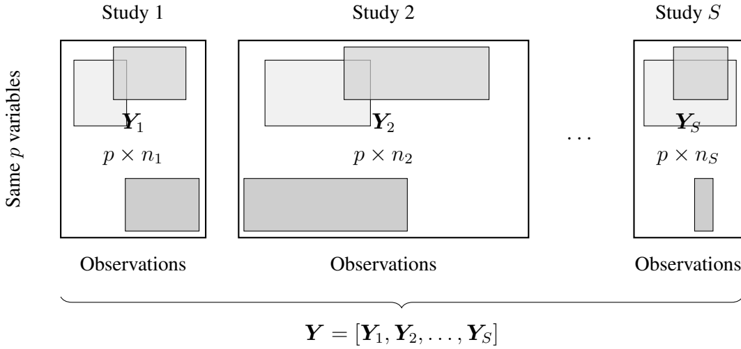
Figure 1: Schematic representation of the multi-study data structure and bicluster configurations. The S studies \mathbf{Y}_1, \dots, \mathbf{Y}_S share the same p variables but may contain different numbers of observations n_s . Within each study, the grey blocks represent distinct biclusters sharing the same variables across studies but spanning different observations. The top two biclusters have overlapping variables, whereas the bottom biclusters are disjoint. Multiple configurations of overlapping and disjoint biclusters may occur across studies.
