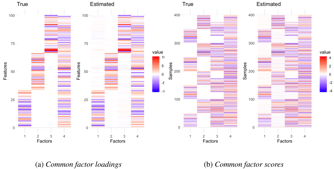
Figure F.1: True and estimated common factor loadings and factor scores for one randomly selected replicate dataset.
