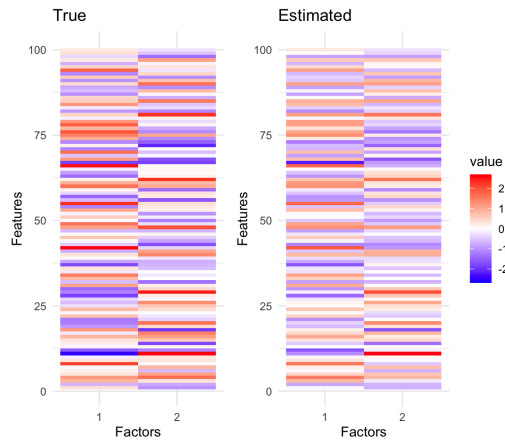
(a) Factor loadings: study 1
