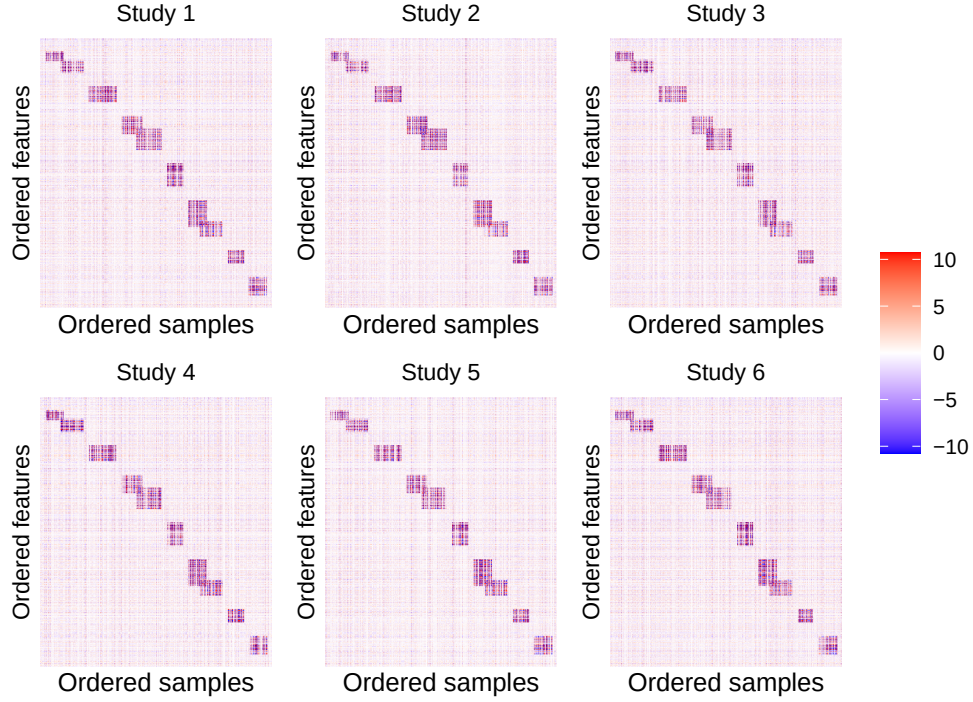
(b) Data matrices reconstructed by the MSFRB model.
