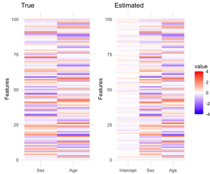
Figure F.3: True and estimated covariate coefficients for one randomly selected replicate dataset.
