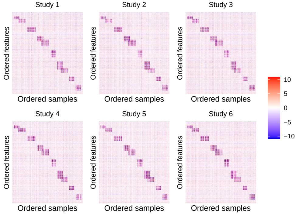
(a) Simulated observed data matrices.
