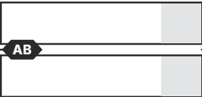
Losers Semi
