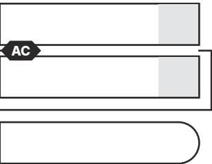
Losers Final
