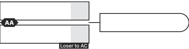
Winners Final
