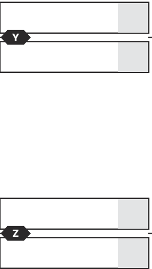
Losers Quarters
