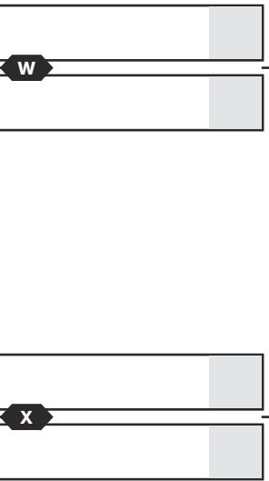
Losers Eighths
