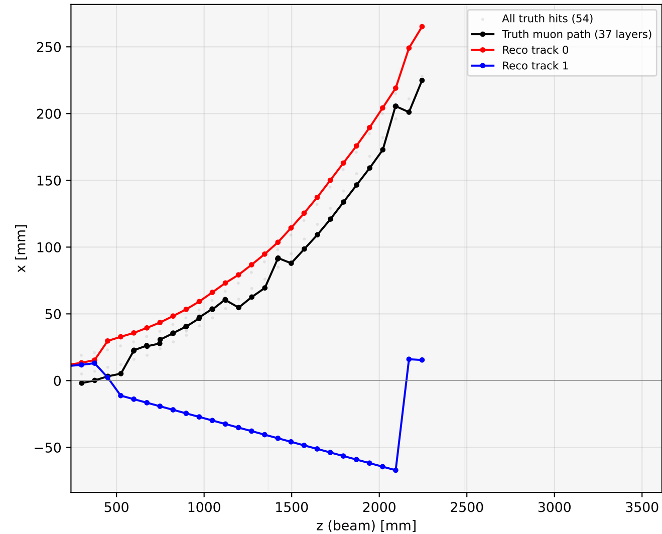
Window 5: MTC z-x (curvature plane)
