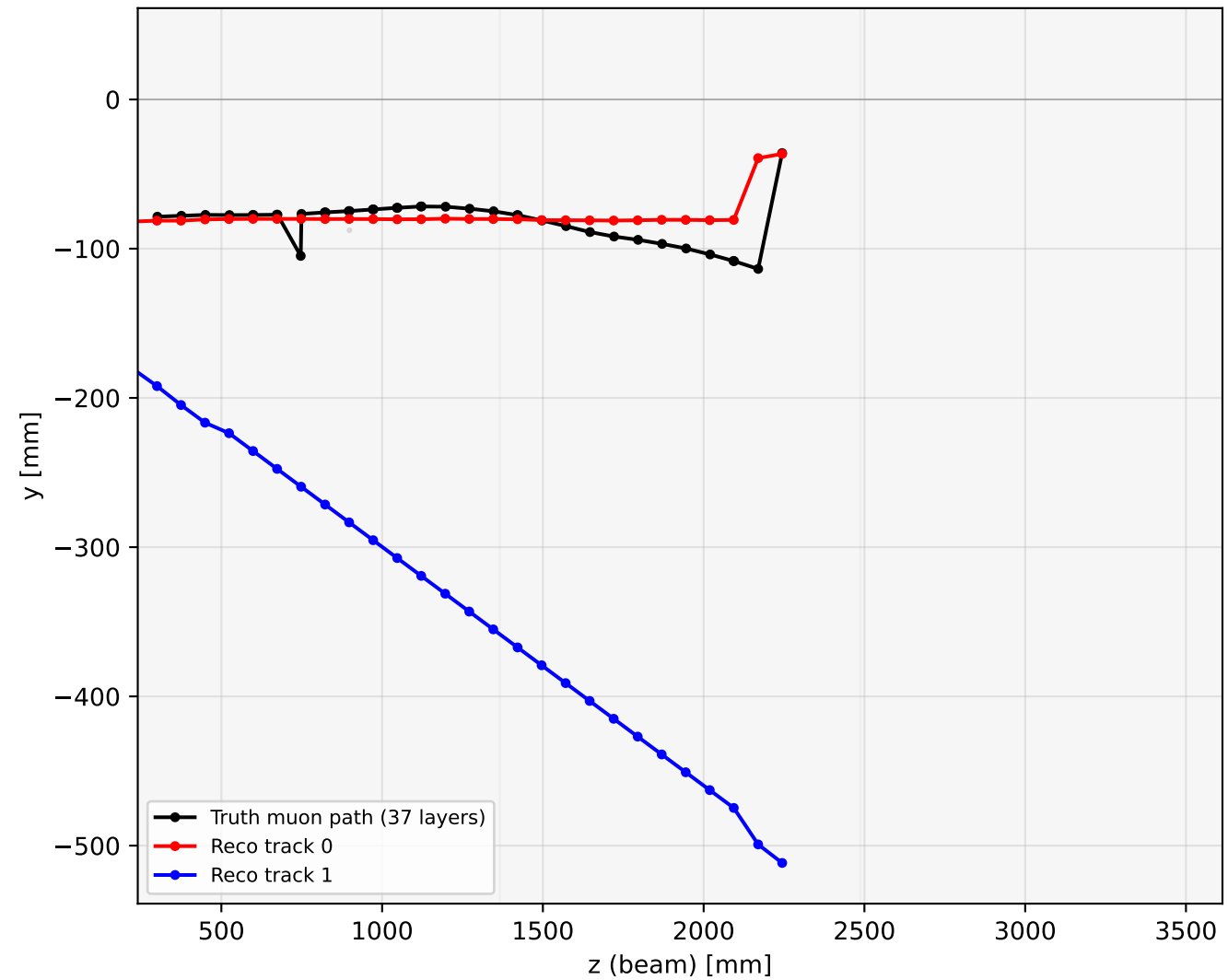
Window 5: MTC z-y
