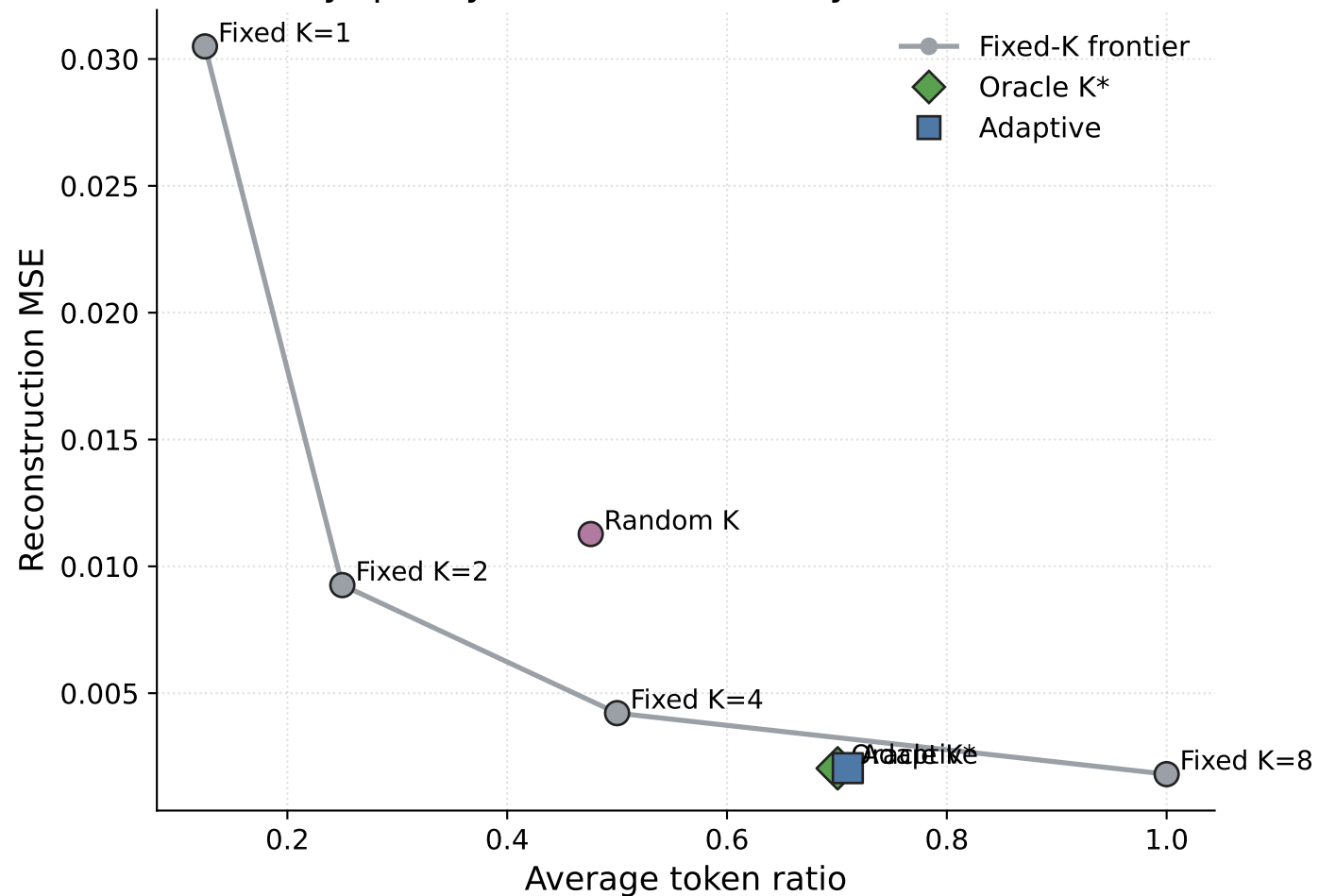
Efficiency-quality trade-off on the synthetic benchmark
