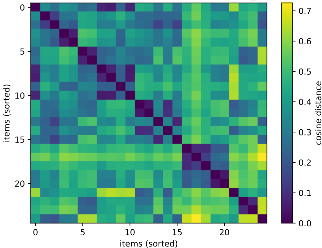
Cosine distance heatmap (sorted by persona_id)
