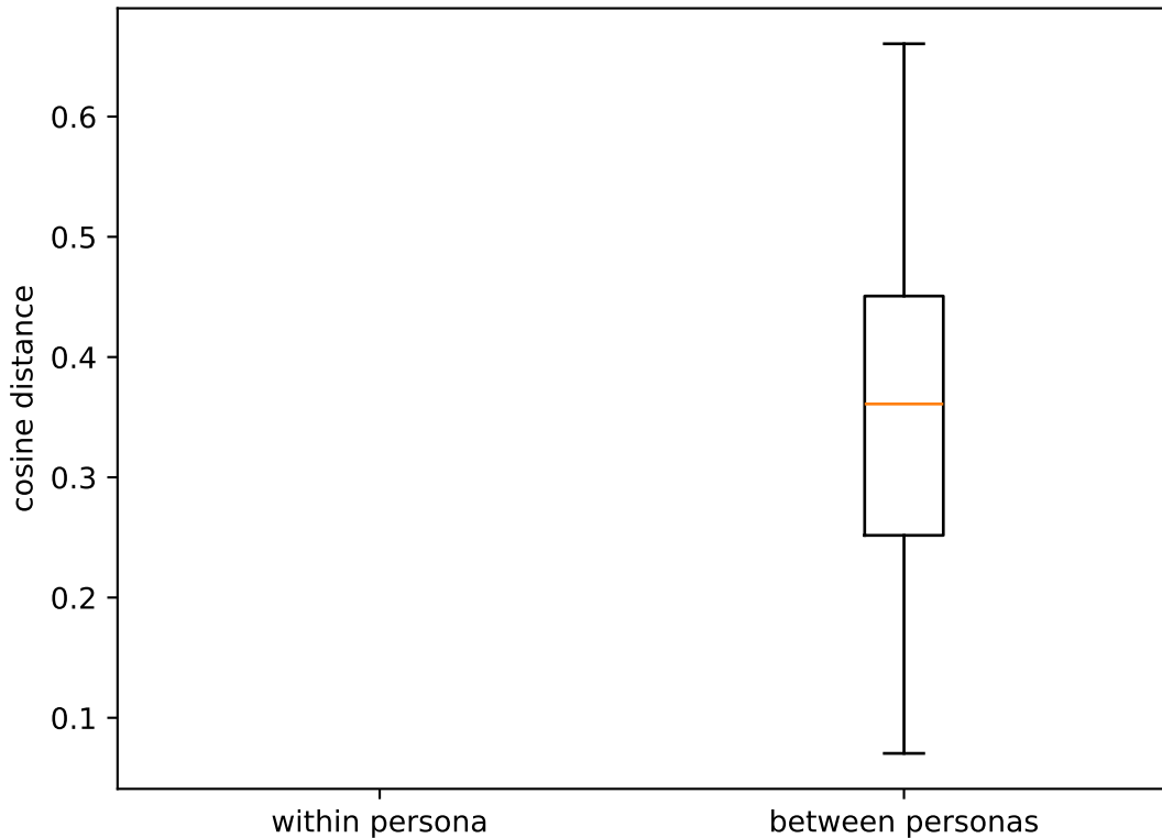
Cosine distances
