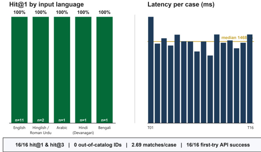
Fig. 3. Grounded-matcher benchmark (16 cases, single annotator). Left: hit@1 by input-language group - English n=11, Hinglish/Roman Urdu n=2, Arabic, Devanagari Hindi and Bengali n=1 each; the sample is not balanced across languages. Right: per-case end-to-end route latency (includes the model-provider round trip) with median line. Footer reports aggregate metrics from the later of the two live endpoint runs.
