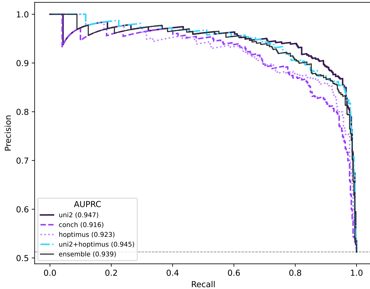
Precision/Recall
