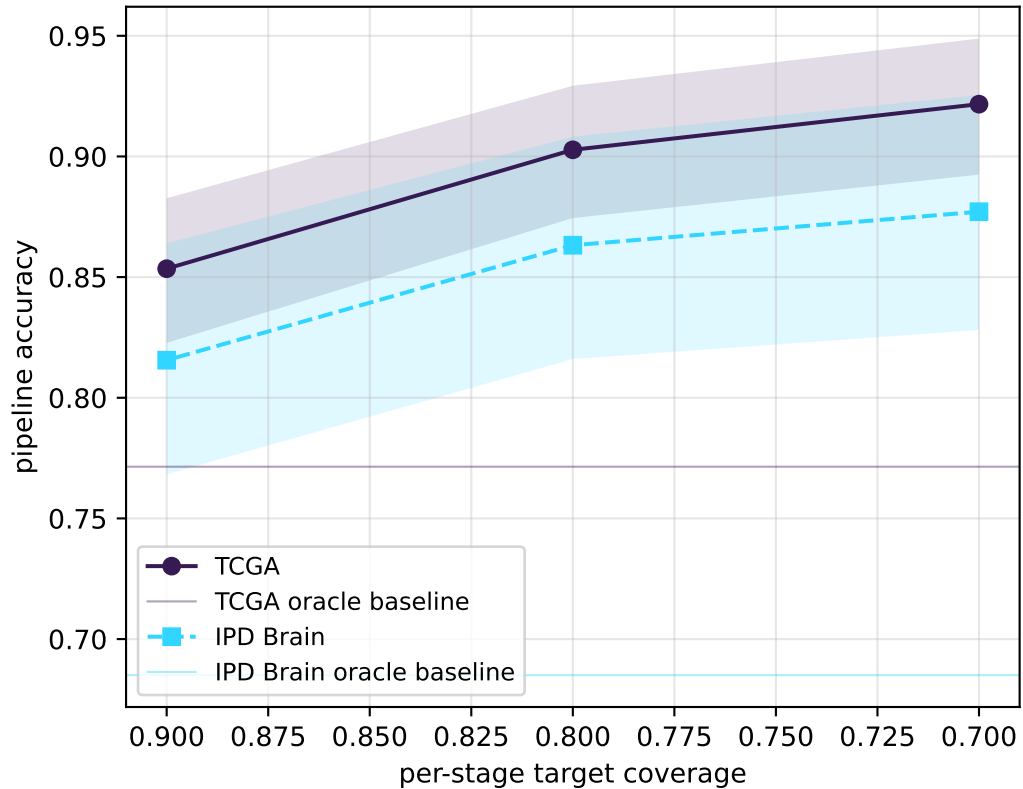
Two-stage pipeline accuracy vs. coverage
