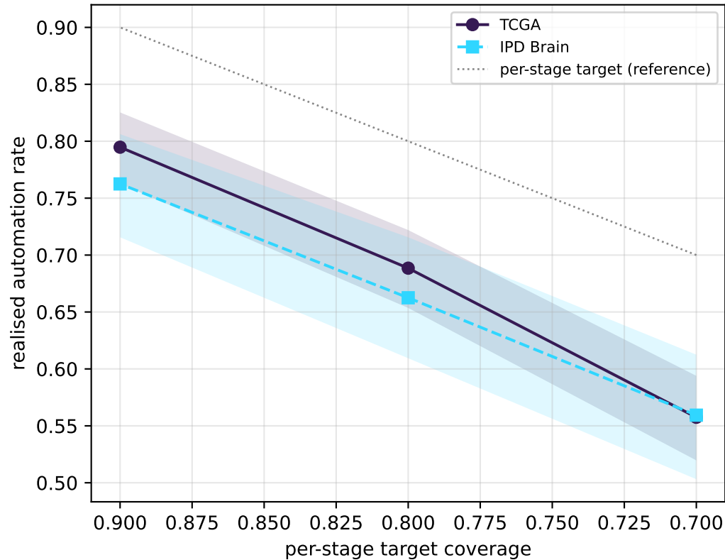
Automation rate vs. coverage
