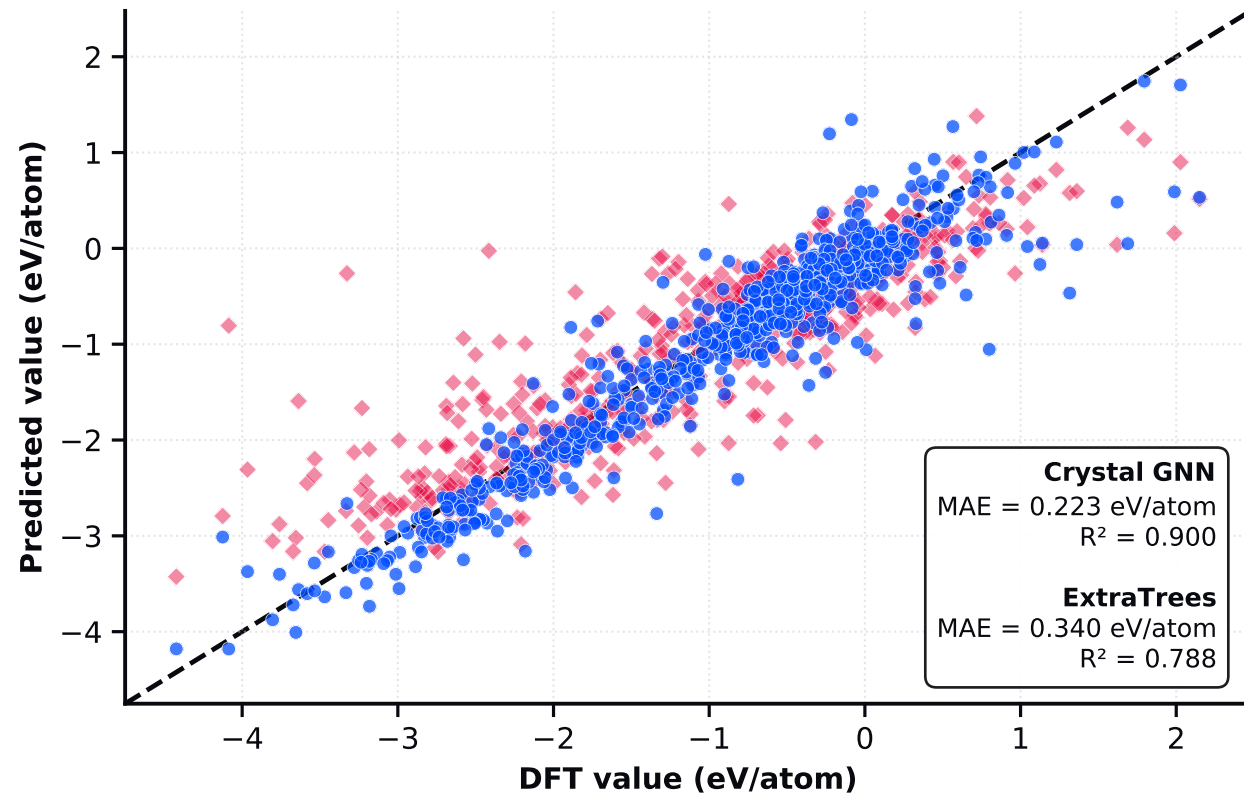
Formation Energy
