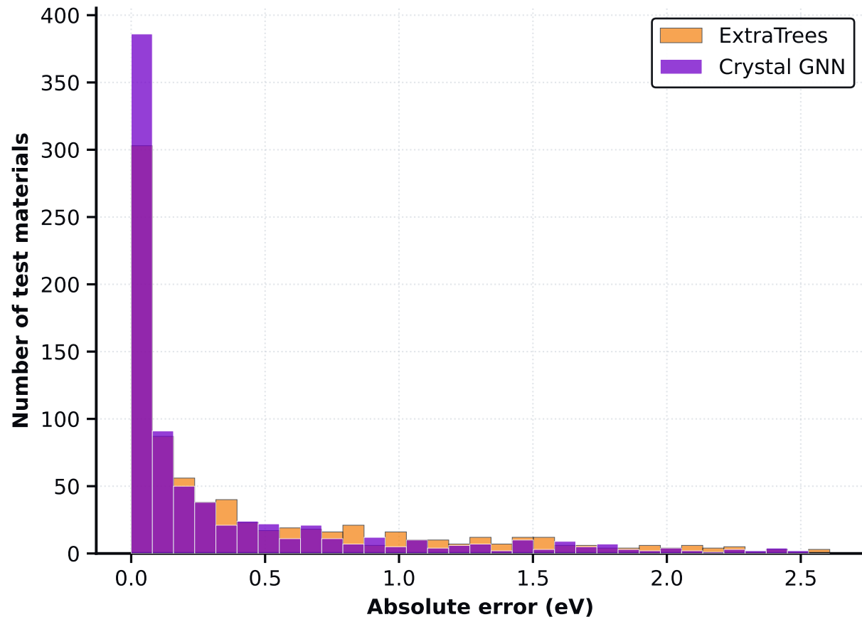
Band-Gap Error
