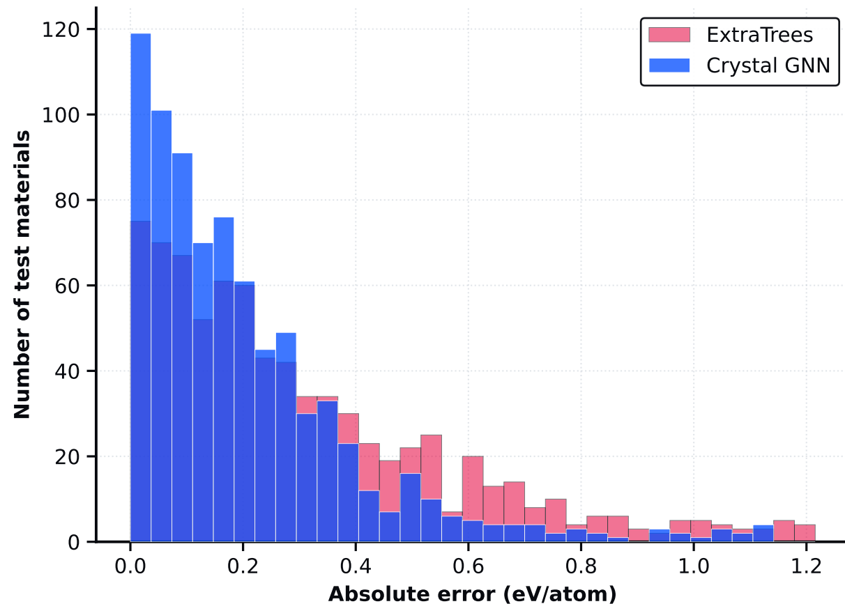
Formation-Energy Error
