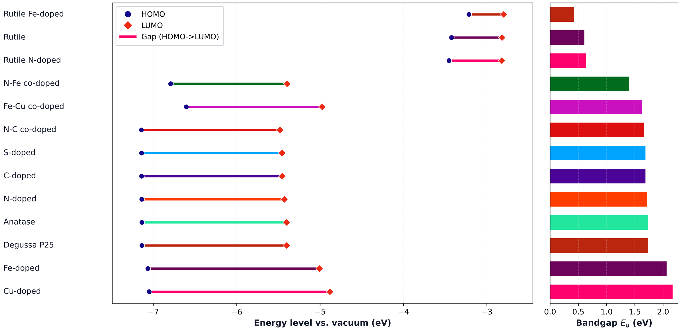
Quantum electronic structure: band alignment & frontier levels
