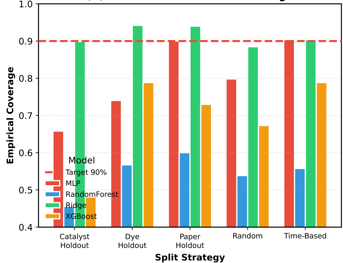
(C) Conformal Prediction Coverage
