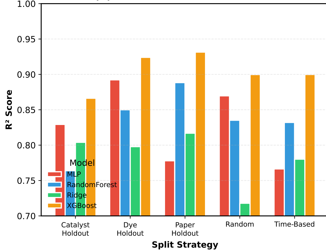
(B) Coefficient of Determination
