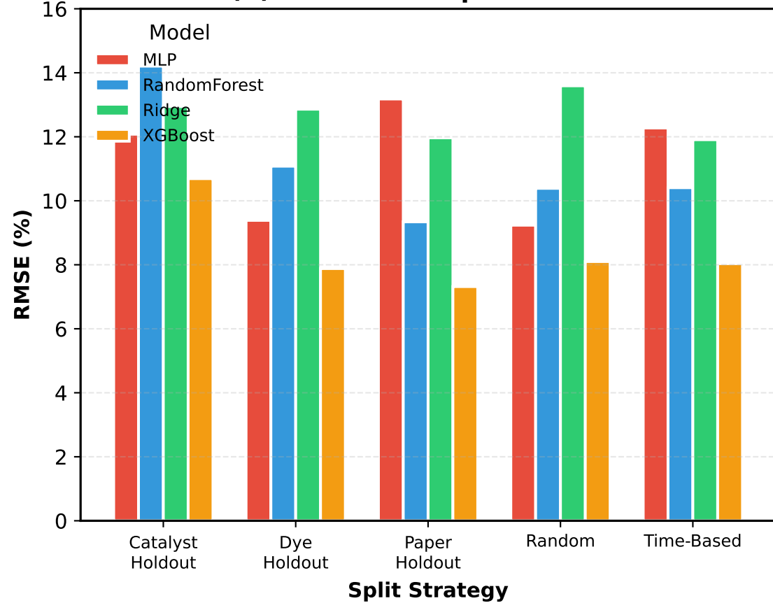
(A) Root Mean Squared Error
