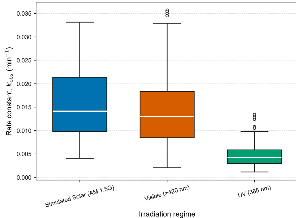
a) Apparent rate constants by light source
