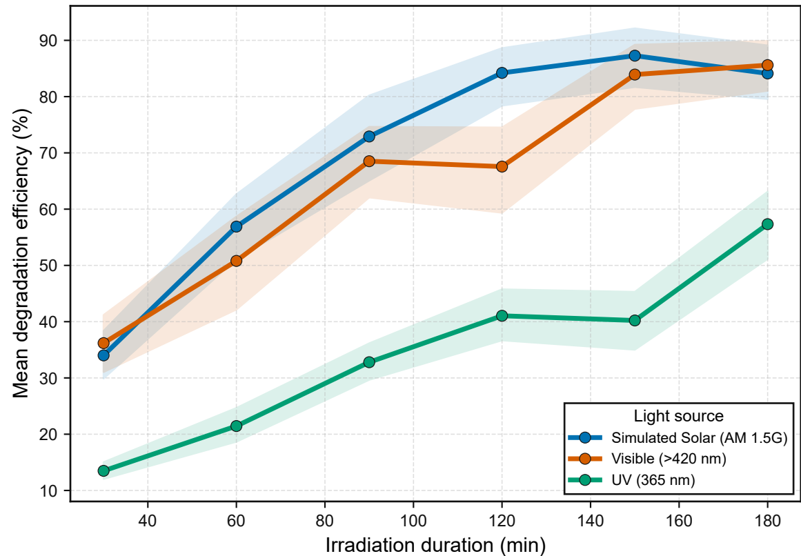
b) Degradation response with irradiation time
