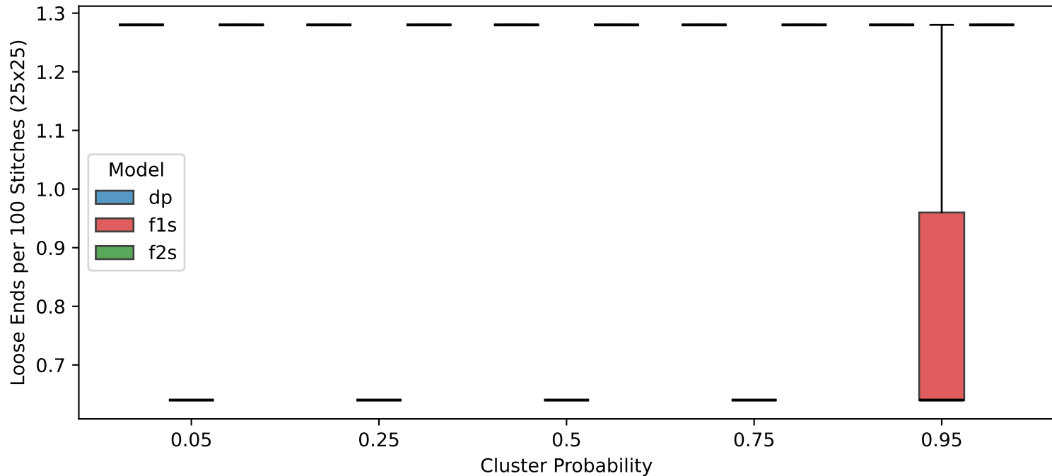
Loose Ends across Cluster Probabilities (25x25)
