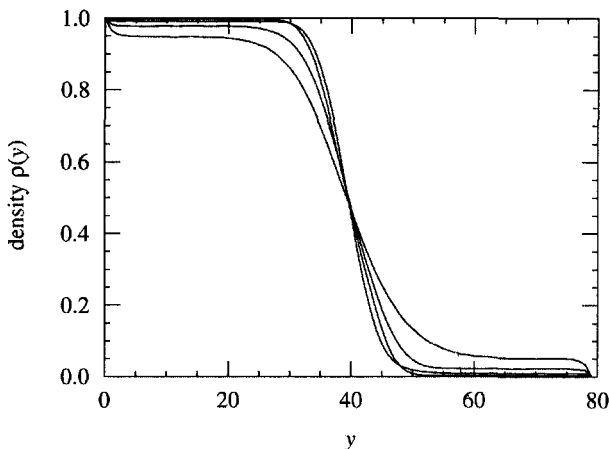
FIGURE 5.3 The average particle density \rho(y) as a function of y for the four simulations shown in Figure 5.2.
