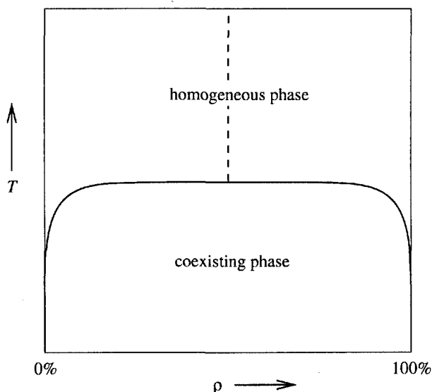
FIGURE 5.1 Phase diagram of the COP Ising model on a square lattice in two dimensions. Depending on the values of the temperature T and density \rho , the system will either be homogeneous or will separate into coexisting domains of the two preferred densities \rho_+ and \rho_- .
