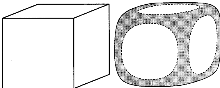
FIGURE 5.6 Schematic depiction of the equilibrium crystal shape for the COP Ising model on a cubic lattice at zero temperature (left) and at a non-zero temperature below the roughening temperature. Above the roughening temperature, the flat facets disappear.
