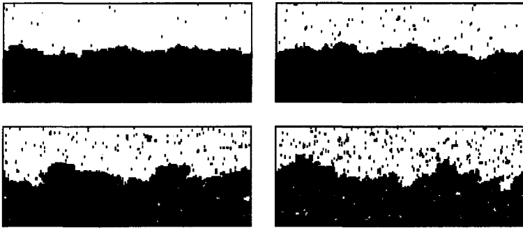
FIGURE 5.2 Typical interface configurations at several temperatures. From top left to bottom right the temperatures are T/T_c=0.6, 0.7, 0.8 , and 0.9 . The interface becomes fuzzier with increasing temperature and at the same time the particle densities \rho_- and \rho_+ approach each other.
