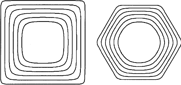
FIGURE 5.5 Equilibrium crystal shapes as a function of temperature on a square lattice (left) and a hexagonal one (right). The outermost droplet shapes correspond to inverse temperatures of \beta J = 9.3 in each case. Going inwards, the values of \beta for the other shapes are factors of 2, 3, 4, 5 and 6 lower. To make the figure clearer we have rescaled the overall size of the droplets so that the different curves do not overlap.
