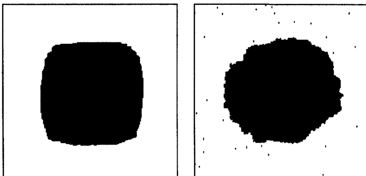
FIGURE 5.4 Typical droplet configurations at T/T_c = 0.25 (left) and T/T_c = 0.5 (right). At low temperatures the boundary of the droplet is quite sharp and the droplet's shape resembles a square. With increasing temperature the boundary becomes fuzzier and the droplet's shape becomes round.
