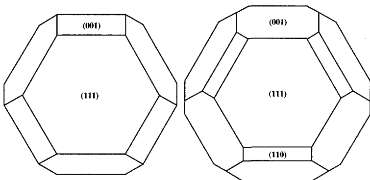
FIGURE 5.7 Equilibrium crystal shape of the COP Ising model on a face-centred cubic lattice at zero temperature without next-nearest-neighbour interactions (left) and after the introduction of small ferromagnetic next-nearest-neighbour interactions (right). After Jayaprakash and Saam (1984).
