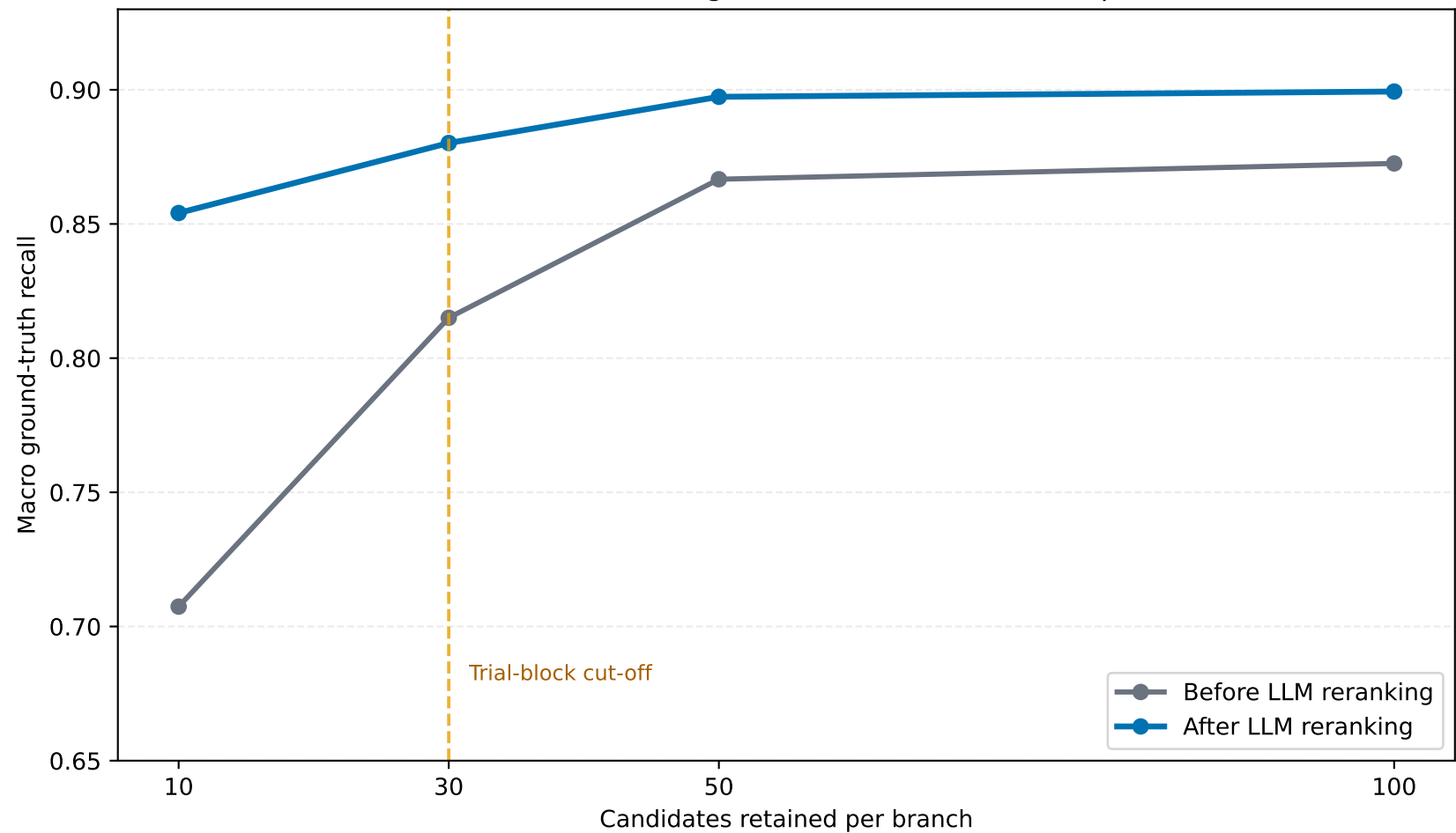
Effect of LLM reranking within fixed A3 candidate pools
