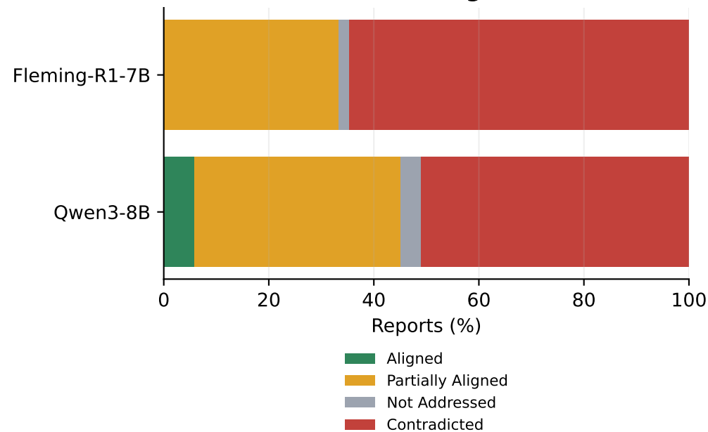
Conclusion alignment
