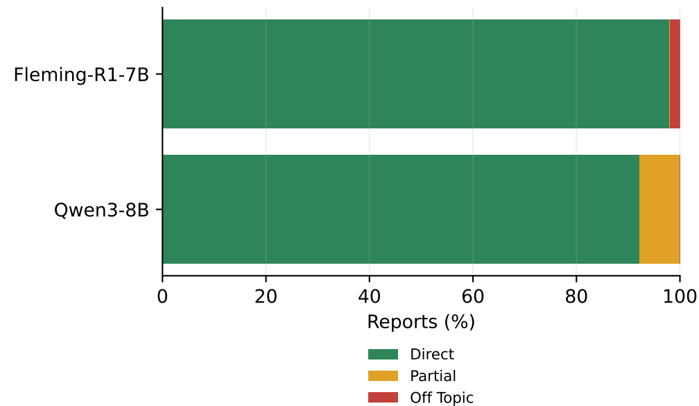
Question relevance
