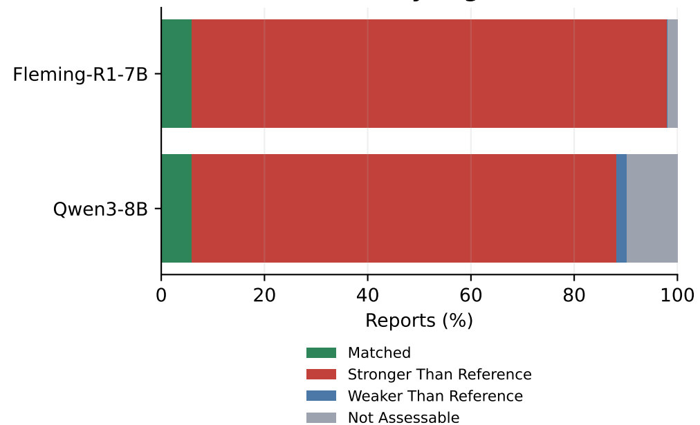
Uncertainty alignment
