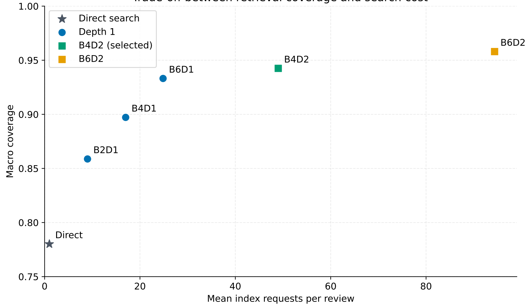
Trade-off between retrieval coverage and search cost
