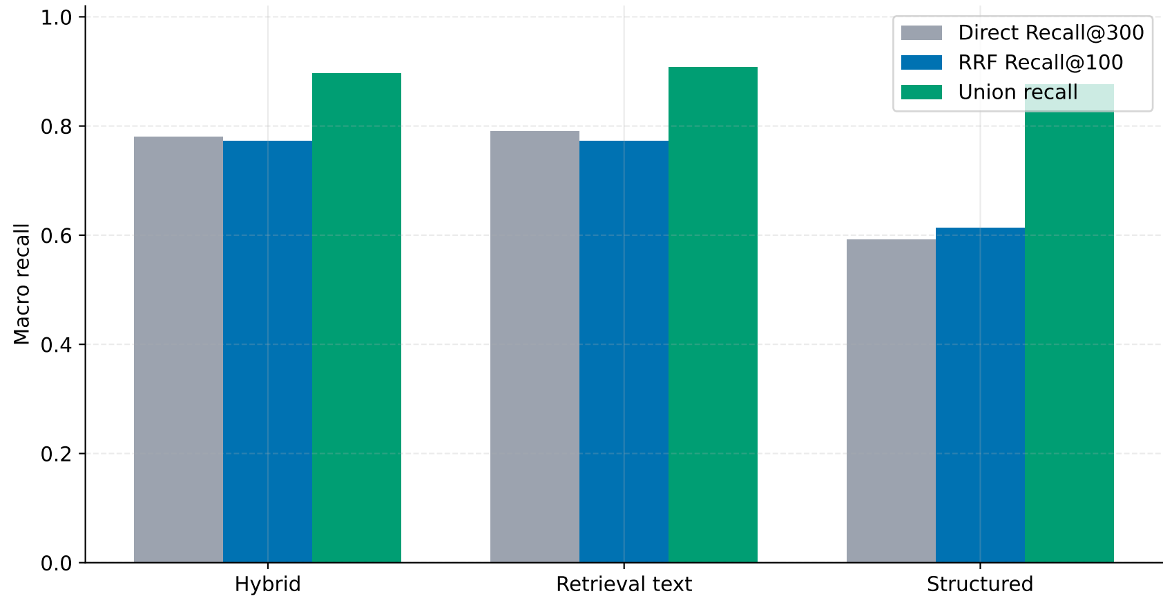
End-to-end retrieval by searchable field representation
