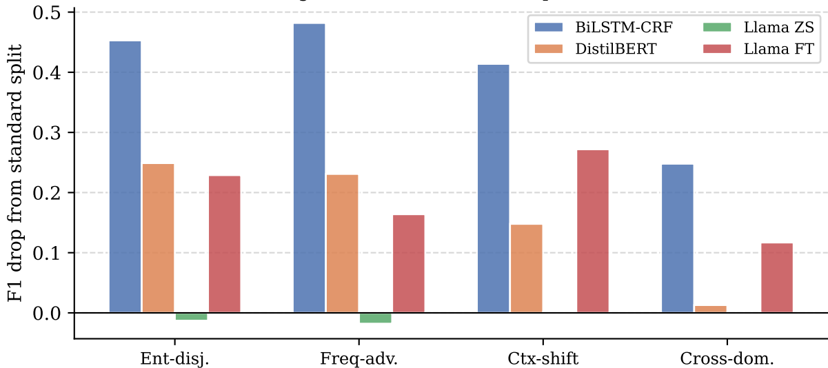
F1 degradation from standard split baseline
