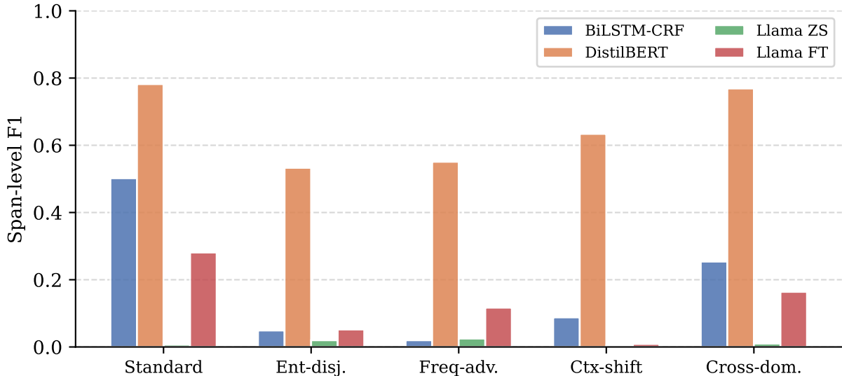
F1 scores across models and evaluation conditions
