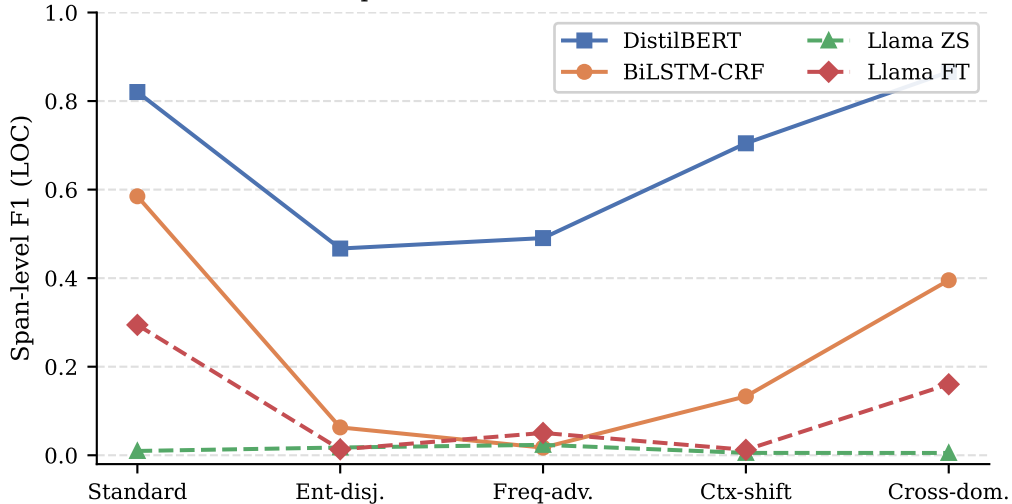
LOC span F1 across evaluation conditions
