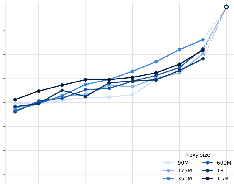
DA-ckpt (reference is the final checkpoint of the same size)
