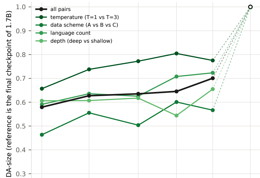
Accuracy → 1.7B accuracy
