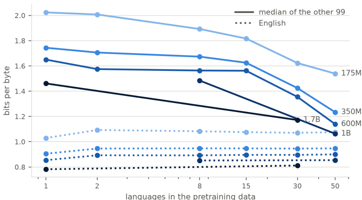
Figure 3. Held-out bits-per-byte at the final checkpoint, deep / scheme A / seed 1904. English pays a one-time cost at the first extra language and nothing after; the non-English median falls throughout.
