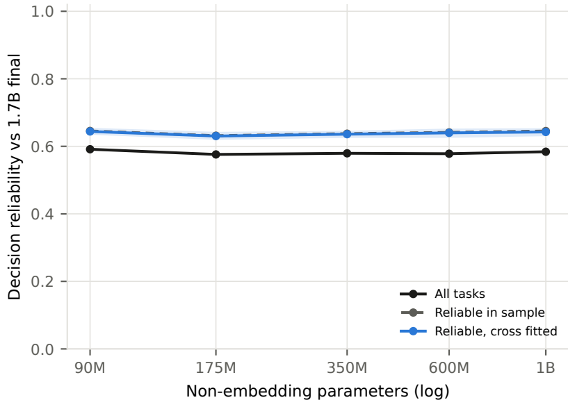
Benchmarks
