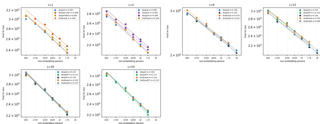
Scaling fit per language setting — every ladder and data scheme overlaid, each fitted separately line fitted WITHOUT the smallest rung then predicting it; red ring = off trend
