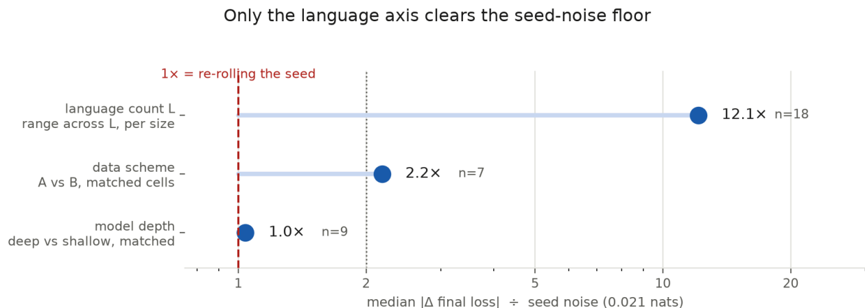
Figure 4. Median |\Delta \text{ final loss}| for each axis, in units of the seed standard deviation (0.021 nats) measured on the six \times 3 cells. Matched pairs only, healthy cells only.
