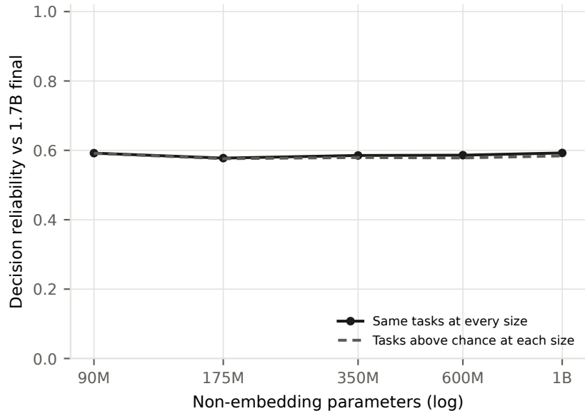
Benchmarks
