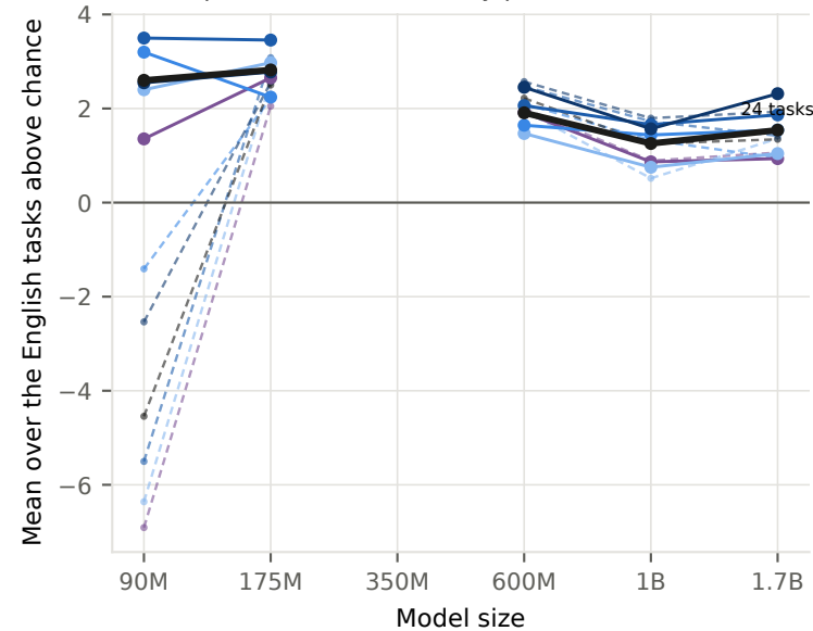
(a) Deep: L1 minus L, accuracy points
