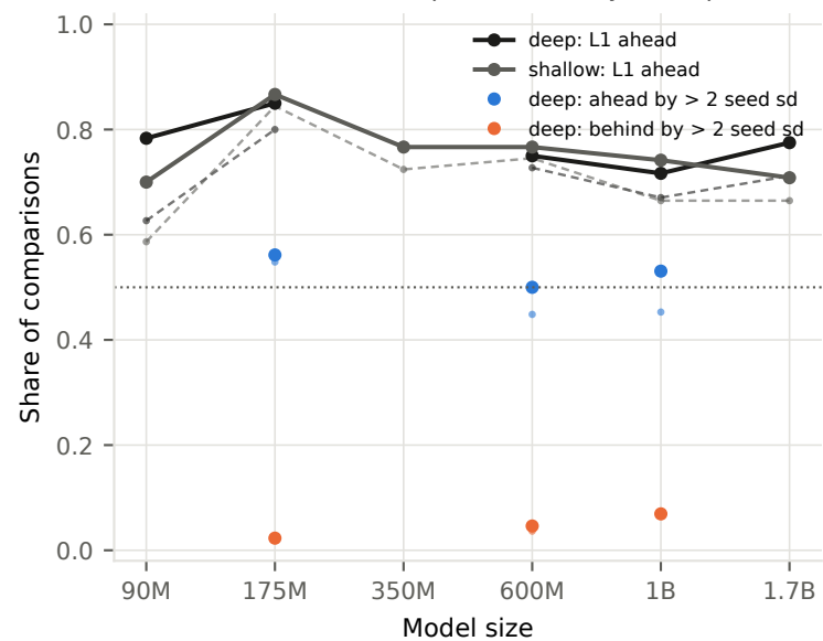
(c) Share of (task, L) comparisons, every L &gt; 1 pooled
