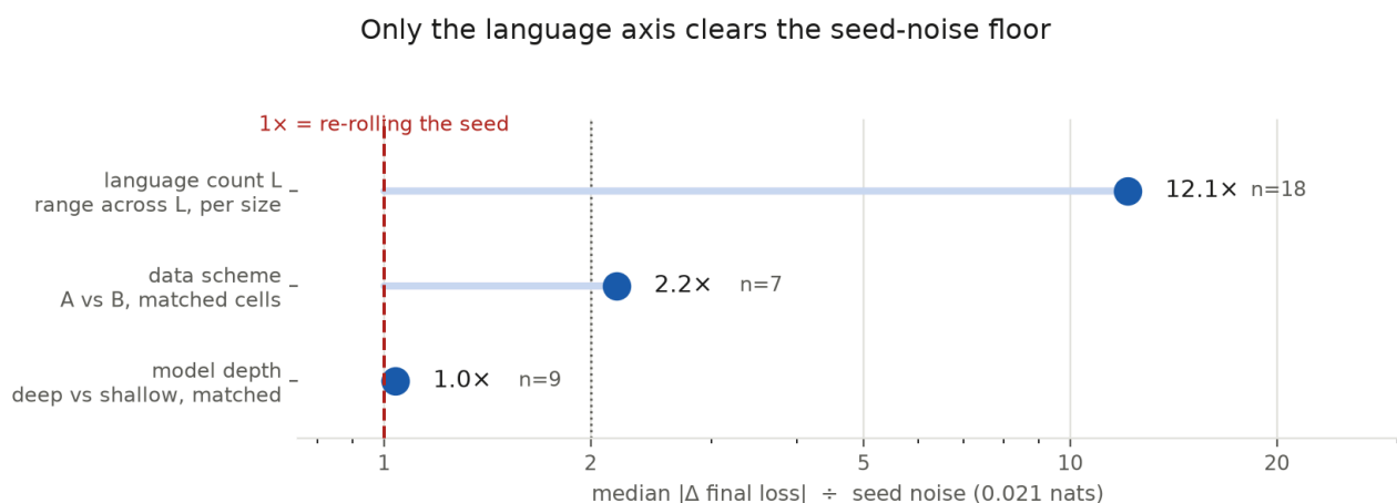
Figure 4. Median |\Delta \text{ final loss}| for each axis, in units of the seed standard deviation (0.021 nats) measured on the six ×3 cells. Matched pairs only, healthy cells only.
