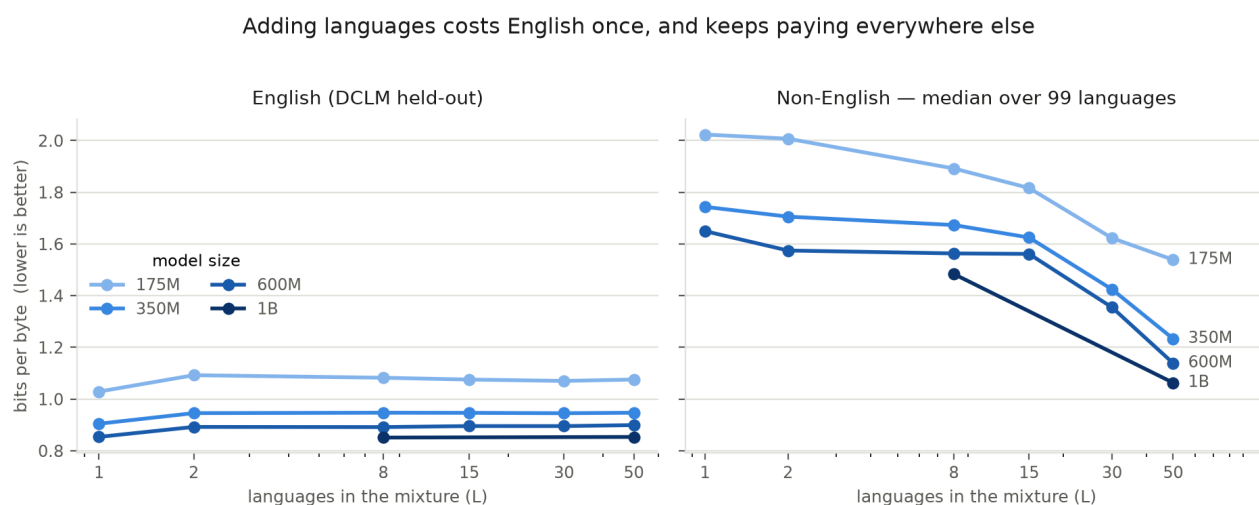
Figure 3. Held-out bits-per-byte at the final checkpoint, deep / scheme A / seed 1904. English pays a one-time cost at the first extra language and nothing after; the non-English median falls throughout.
