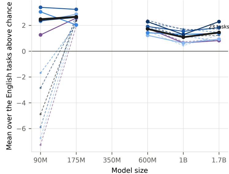
(a) Deep: L1 minus L, accuracy points
