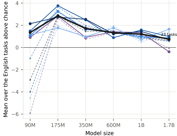
(b) Shallow: L1 minus L, accuracy points
