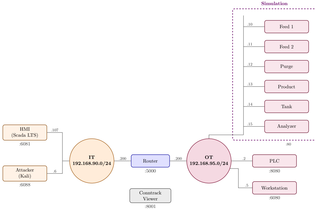
FIGURE 3.1: GRFICSv3 Network Diagram
