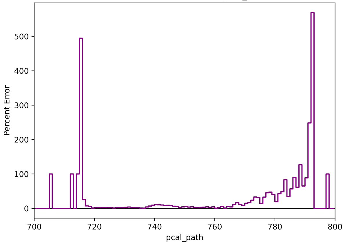
Percent Error: Data vs MC (pcal_path)
