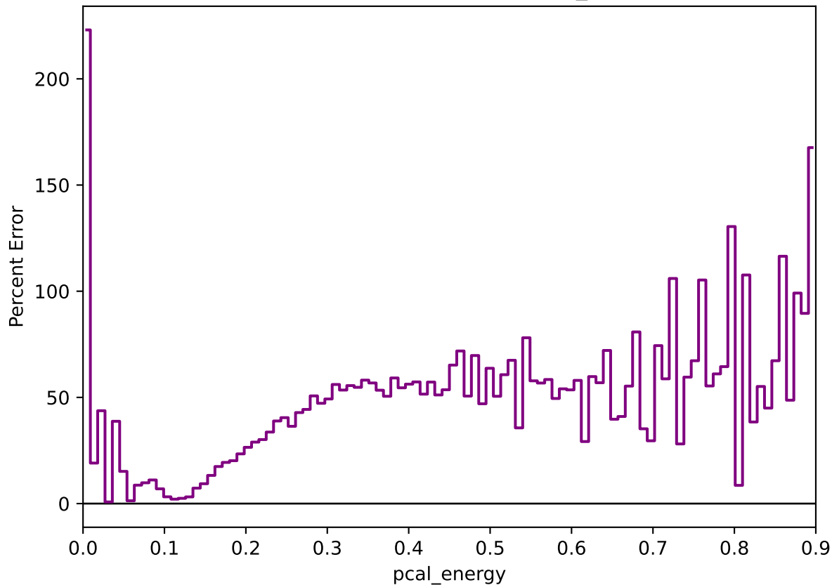
Percent Error: Data vs MC (pcal_energy)
