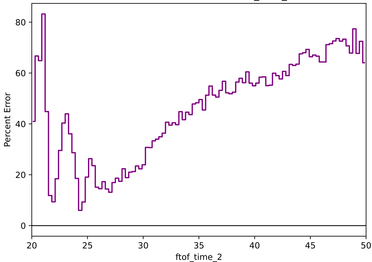
Percent Error: Data vs MC (ftof_time_2)
