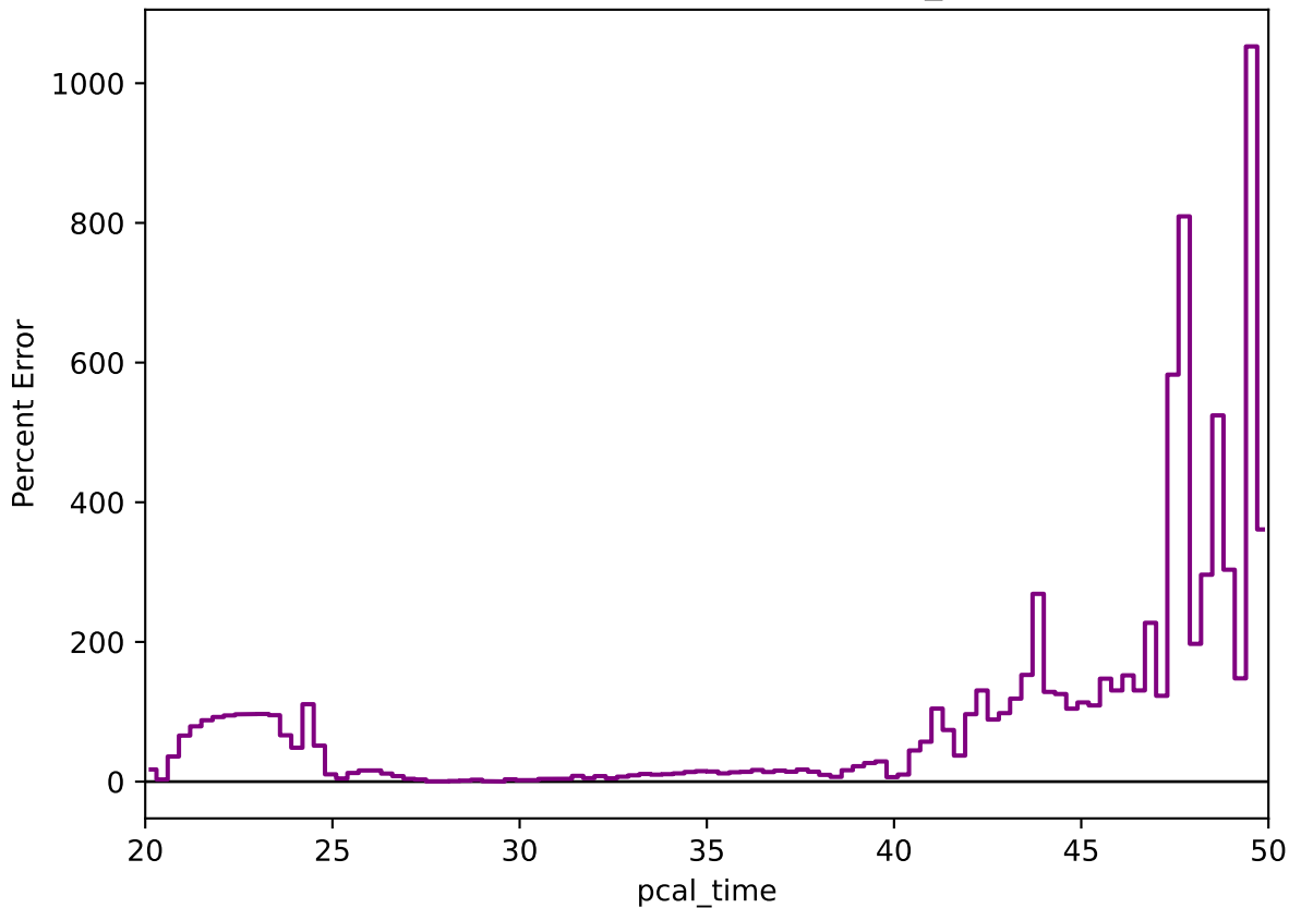
Percent Error: Data vs MC (pcal_time)
