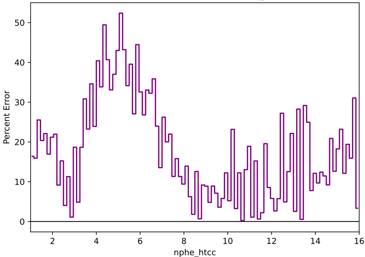
Percent Error: Data vs MC (nphe_htcc)
