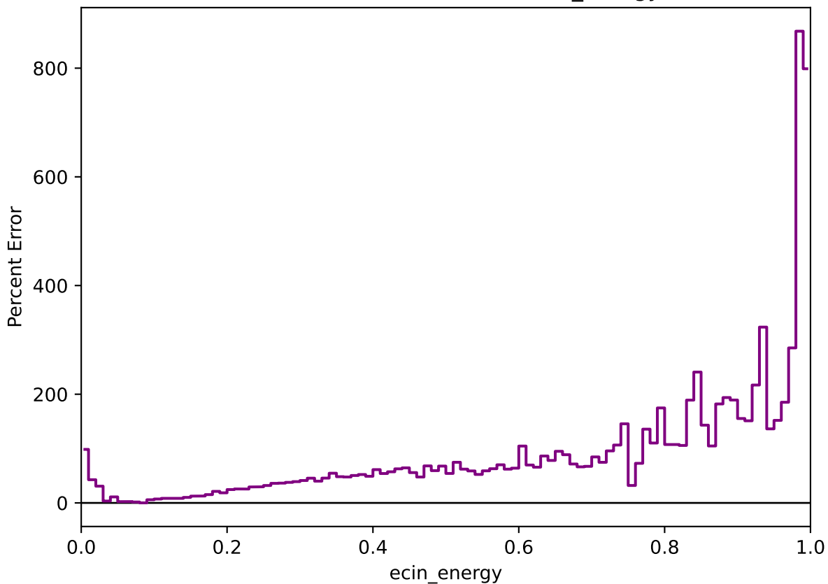
Percent Error: Data vs MC (ecin_energy)
