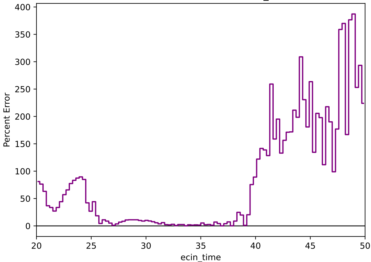
Percent Error: Data vs MC (ecin_time)
