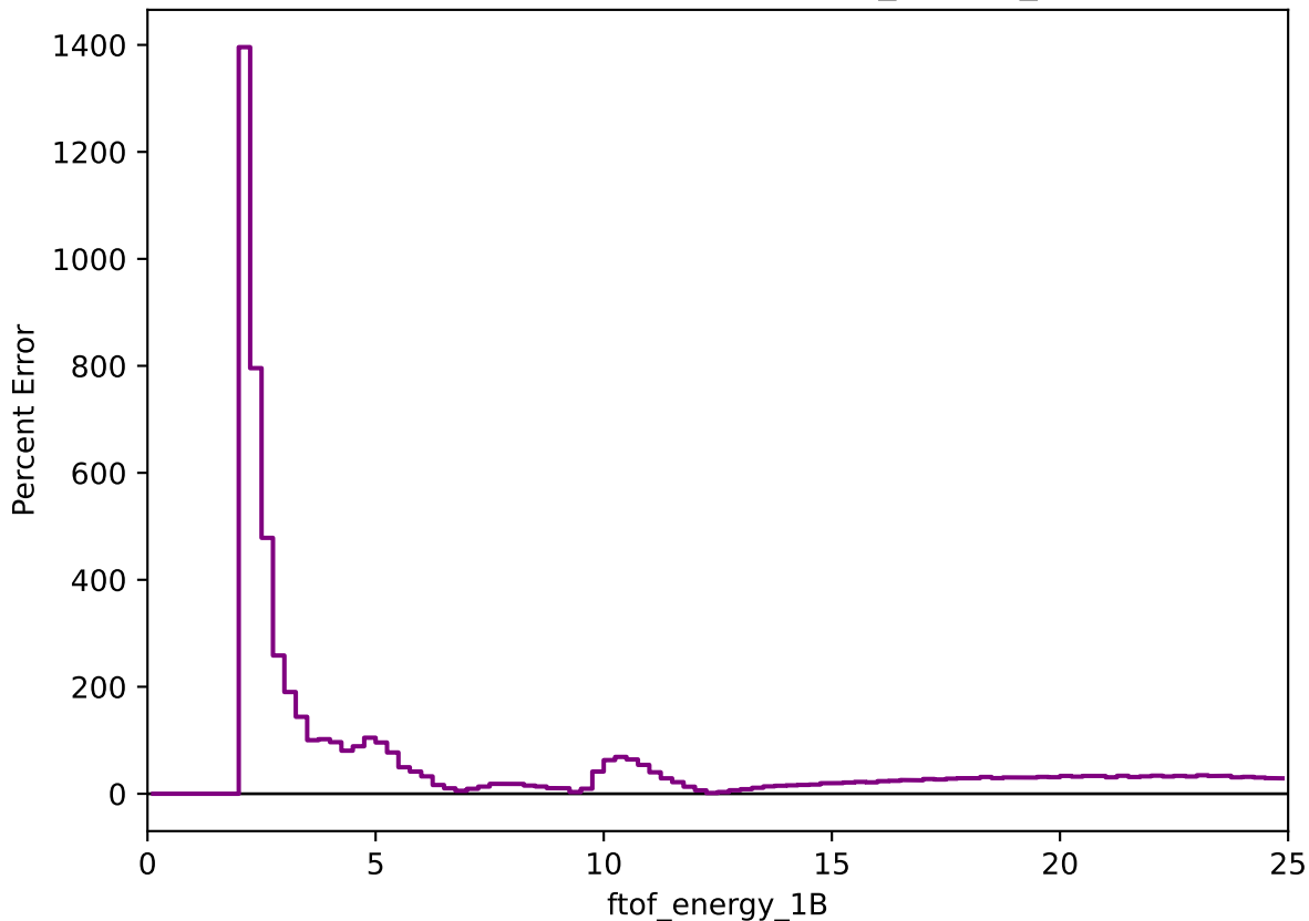
Percent Error: Data vs MC (ftof_energy_1B)
