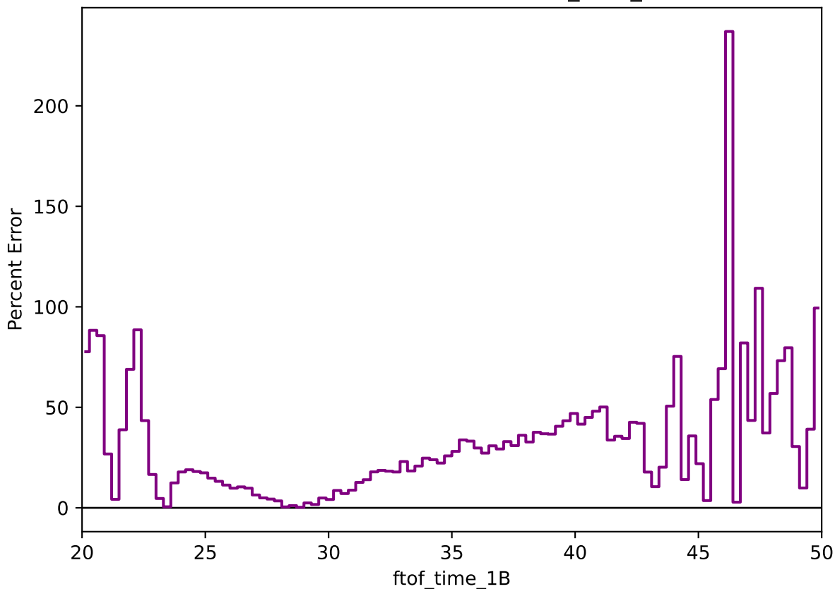
Percent Error: Data vs MC (ftof_time_1B)
