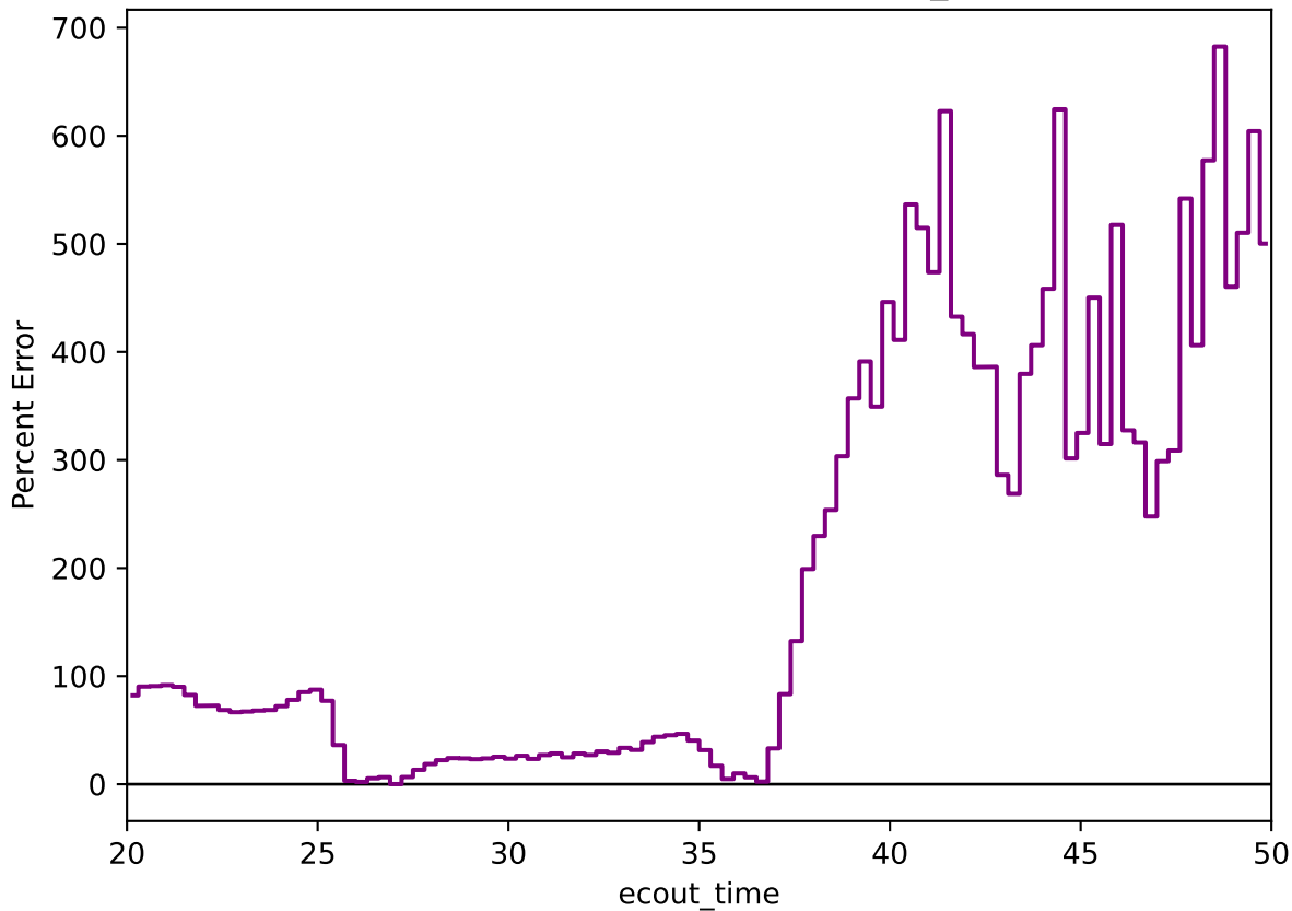
Percent Error: Data vs MC (ecout_time)
