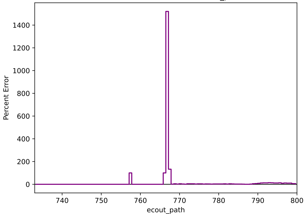
Percent Error: Data vs MC (ecout_path)
