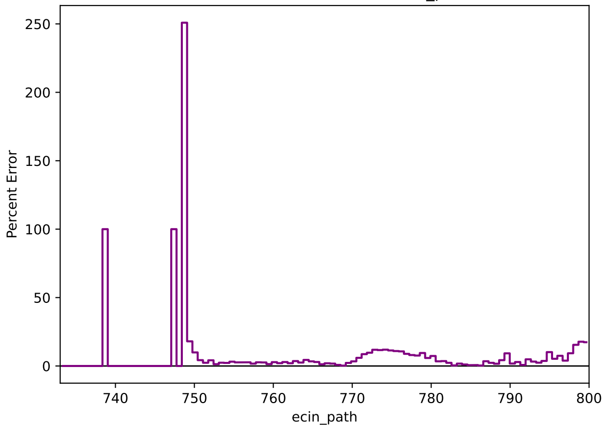
Percent Error: Data vs MC (ecin_path)
