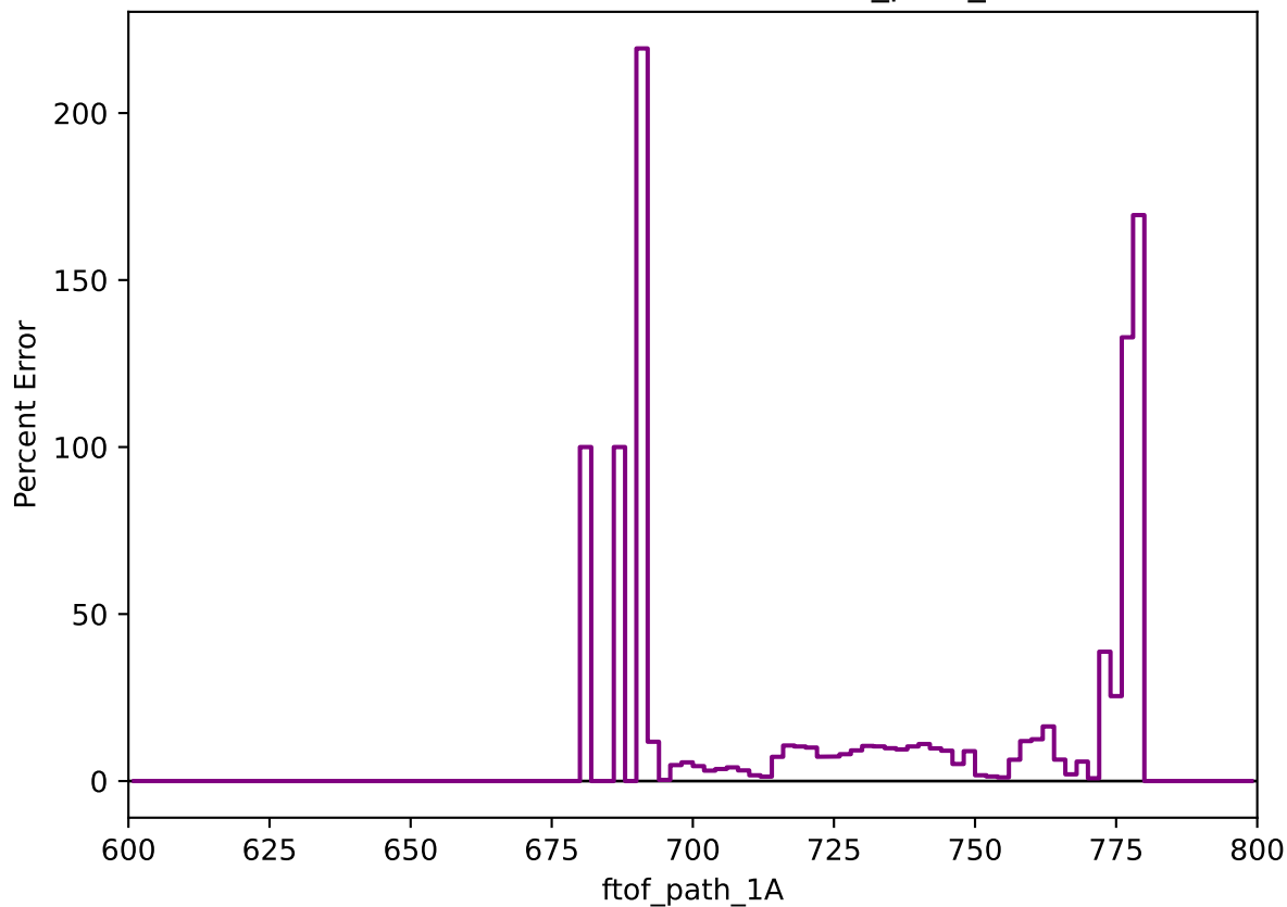
Percent Error: Data vs MC (ftof_path_1A)
