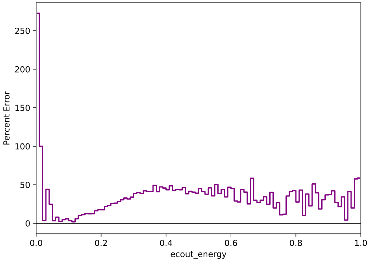
Percent Error: Data vs MC (ecout_energy)
