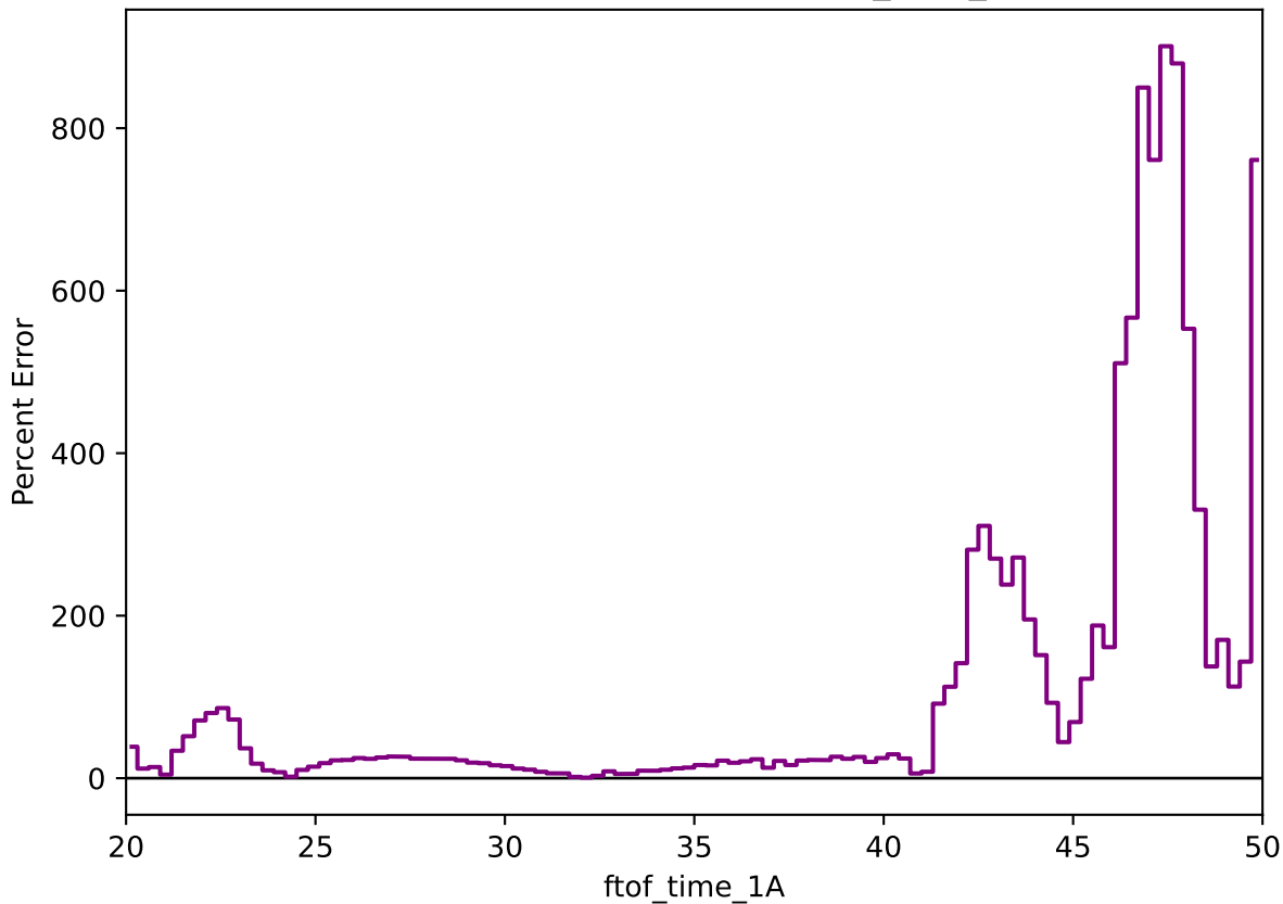
Percent Error: Data vs MC (ftof_time_1A)
