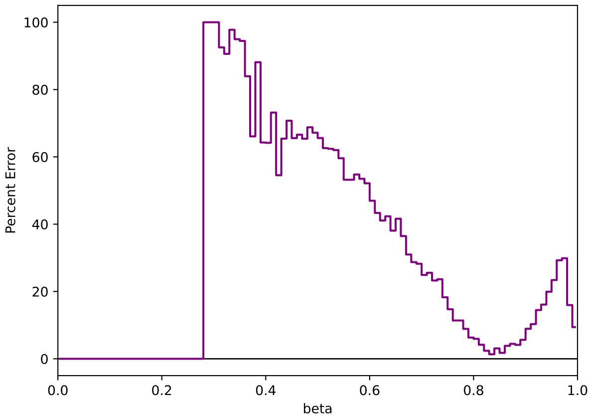
Percent Error: Data vs MC (beta)
