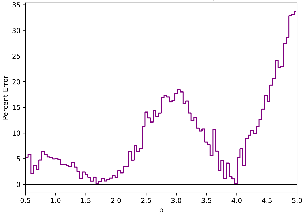
Percent Error: Data vs MC (p)
