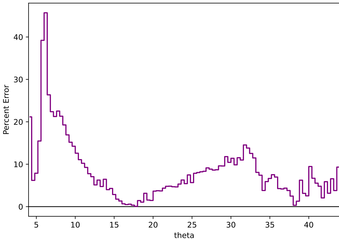
Percent Error: Data vs MC (theta)
