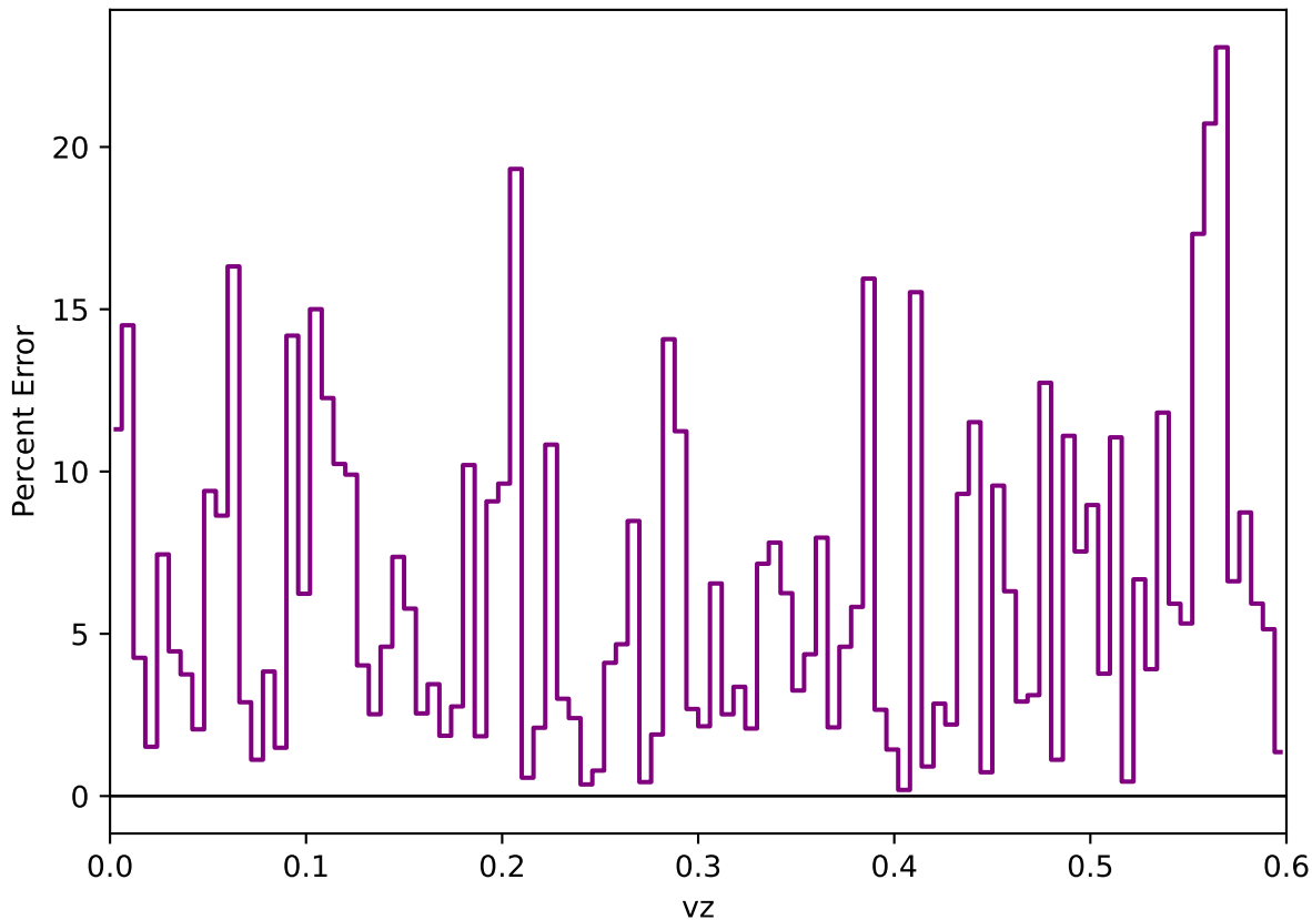
Percent Error: Data vs MC (vz)
