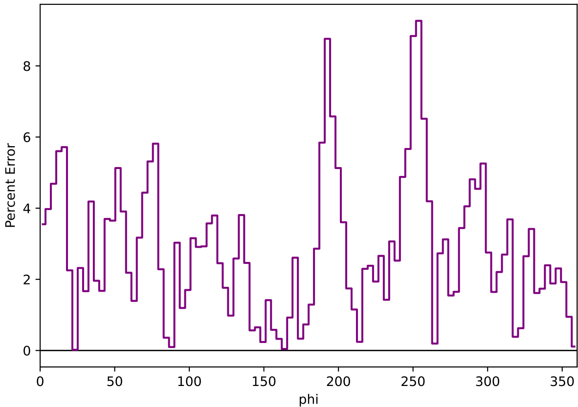
Percent Error: Data vs MC ( \phi )
