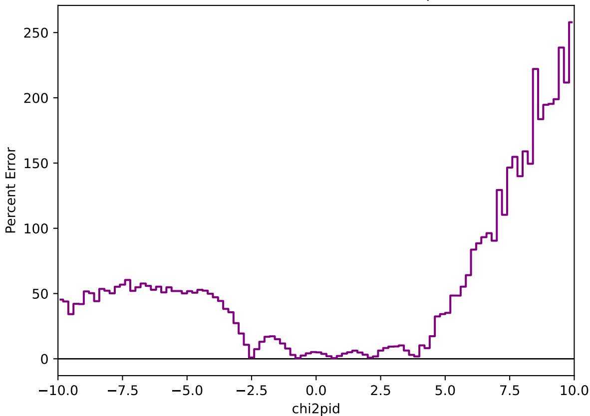
Percent Error: Data vs MC (chi2pid)
