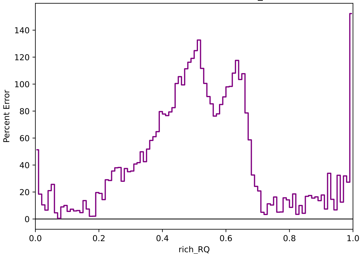
Percent Error: Data vs MC (rich_RQ)
