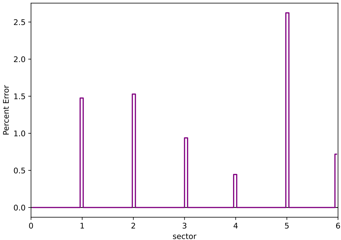
Percent Error: Data vs MC (sector)
