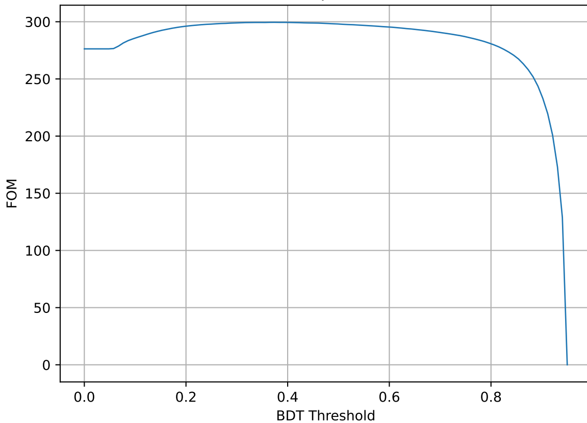
FOM vs Threshold 11.0 < \theta < 17.0 2.75 < p < 3.20
