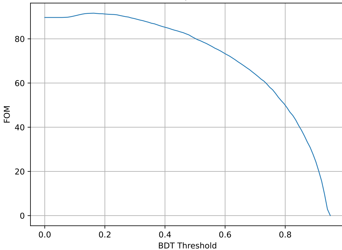
FOM vs Threshold 11.0 < \theta < 17.0 4.55 < p < 5.00
