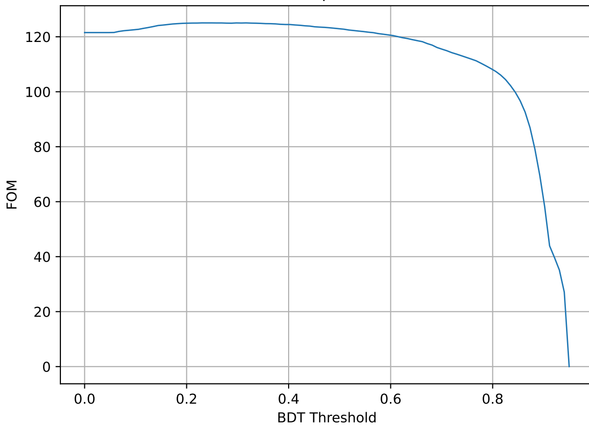
FOM vs Threshold 29.0 < \theta < 35.0 2.30 < p < 2.75
