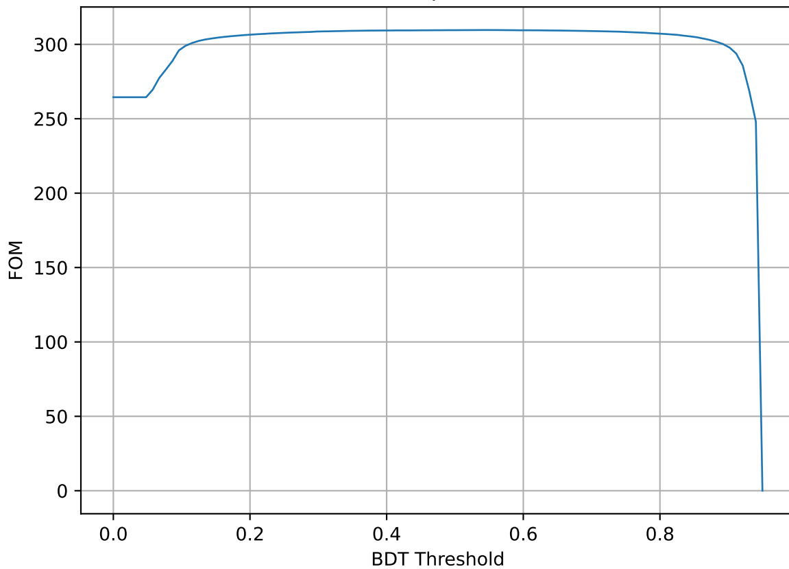
FOM vs Threshold 17.0 < \theta < 23.0 0.95 < p < 1.40
