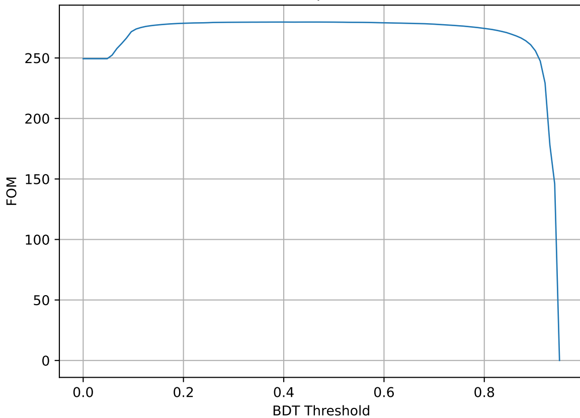
FOM vs Threshold 23.0 < \theta < 29.0 0.95 < p < 1.40
