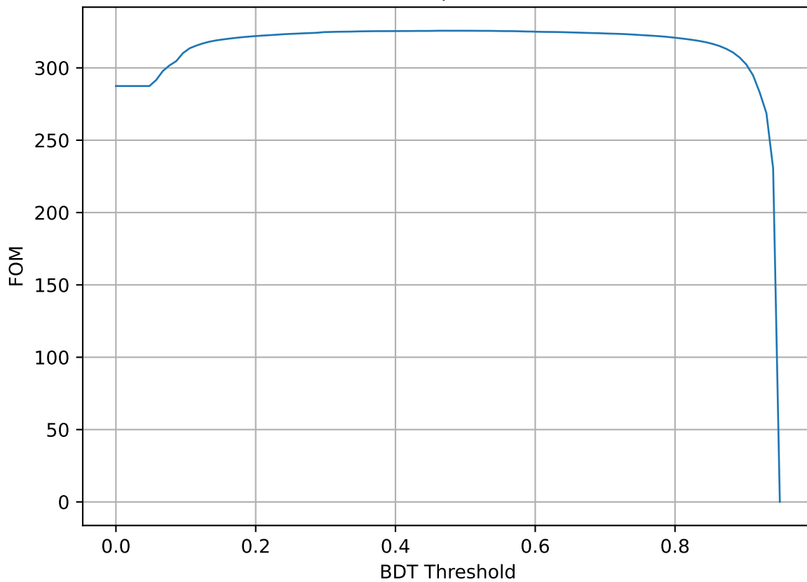
FOM vs Threshold 11.0 < \theta < 17.0 1.40 < p < 1.85
