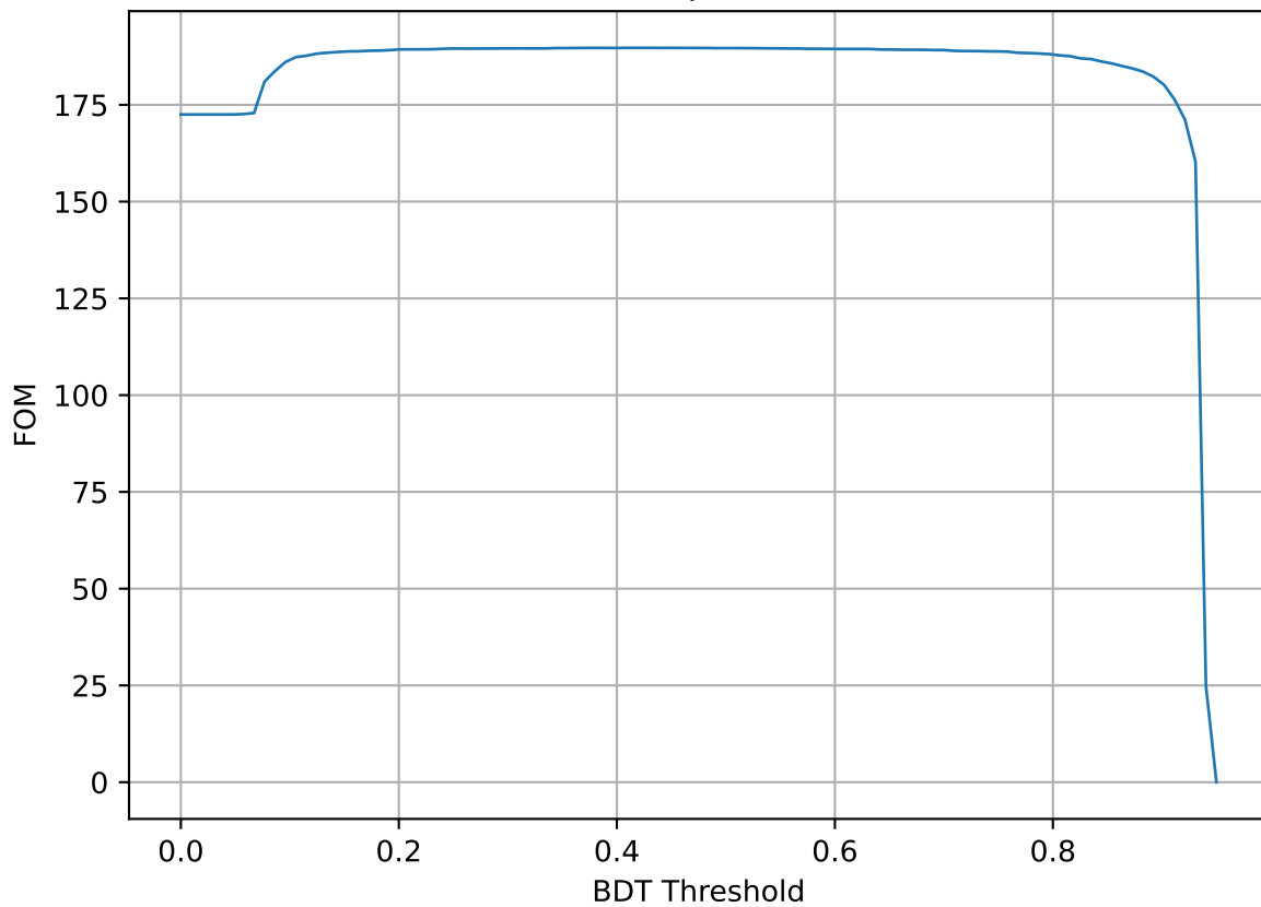
FOM vs Threshold 29.0 < \theta < 35.0 0.50 < p < 0.95
