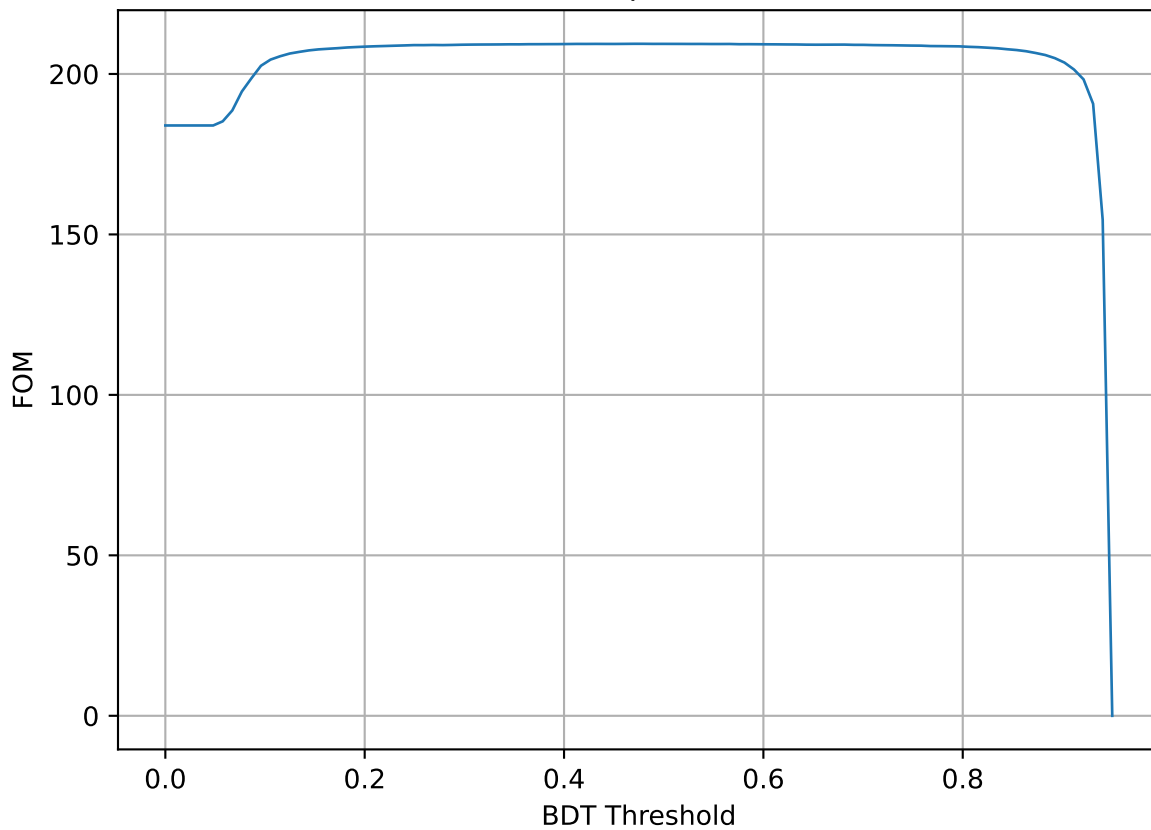
FOM vs Threshold 17.0 < \theta < 23.0 0.50 < p < 0.95
