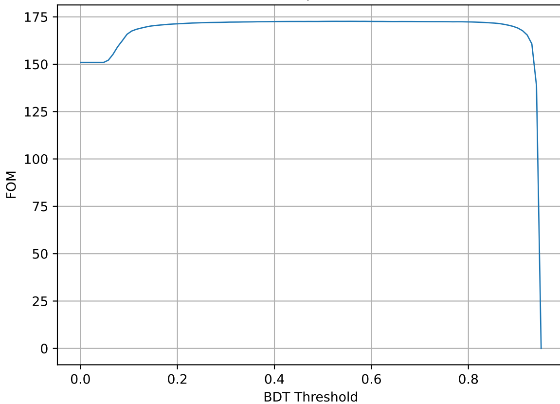
FOM vs Threshold 11.0 < \theta < 17.0 0.50 < p < 0.95
