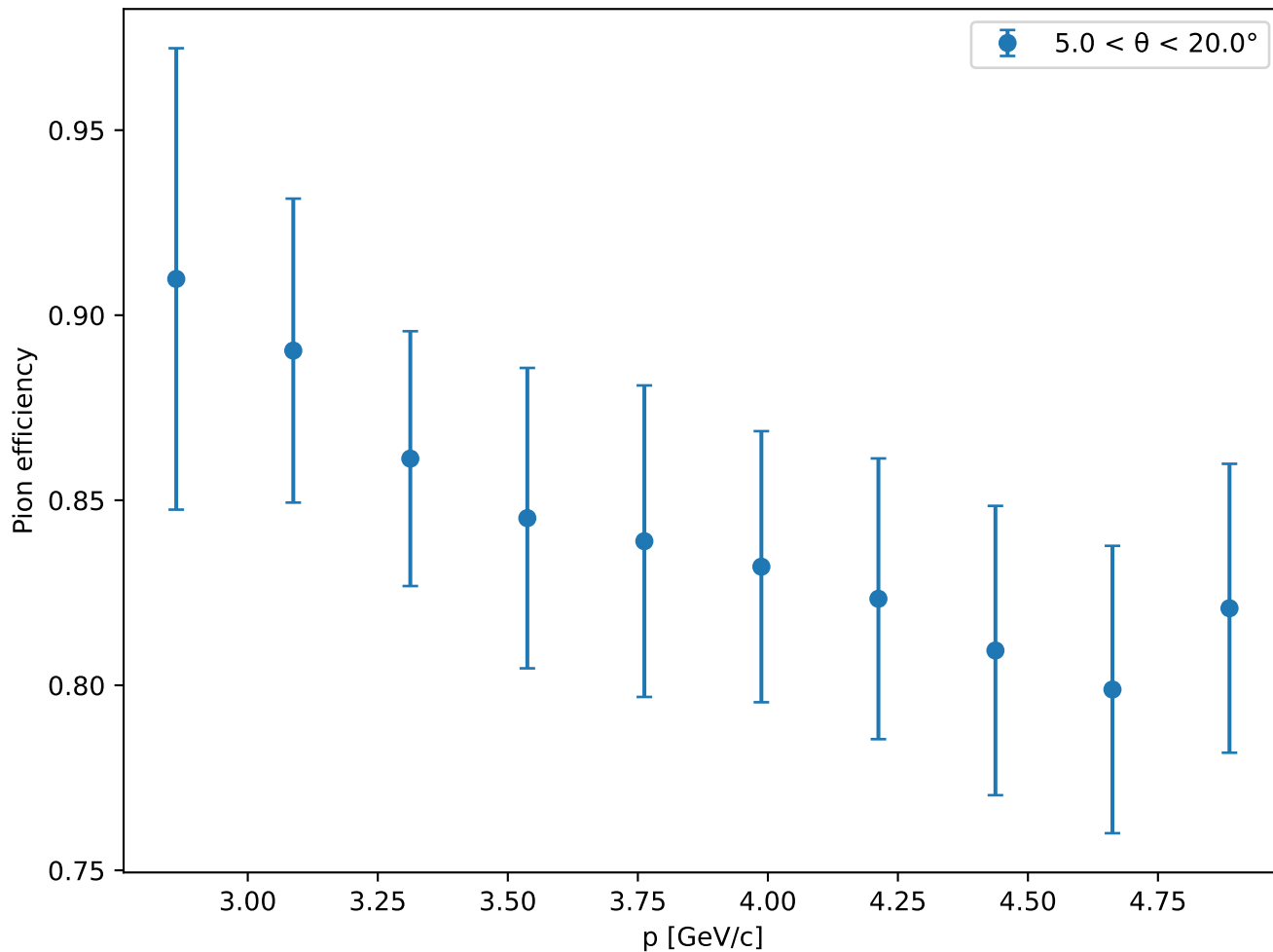
\pi Efficiency vs Momentum
