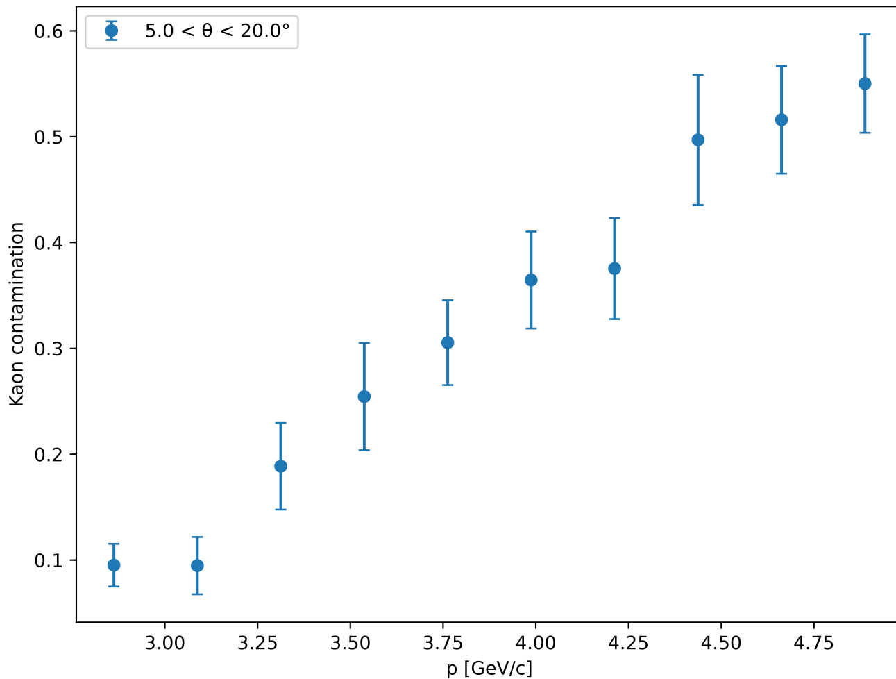
SIDIS Kaon Contamination vs Momentum
