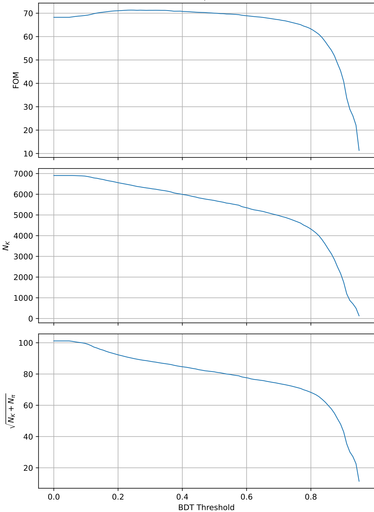
FOM vs Threshold 29.0 < theta < 35.0 2.66 < p < 2.93
