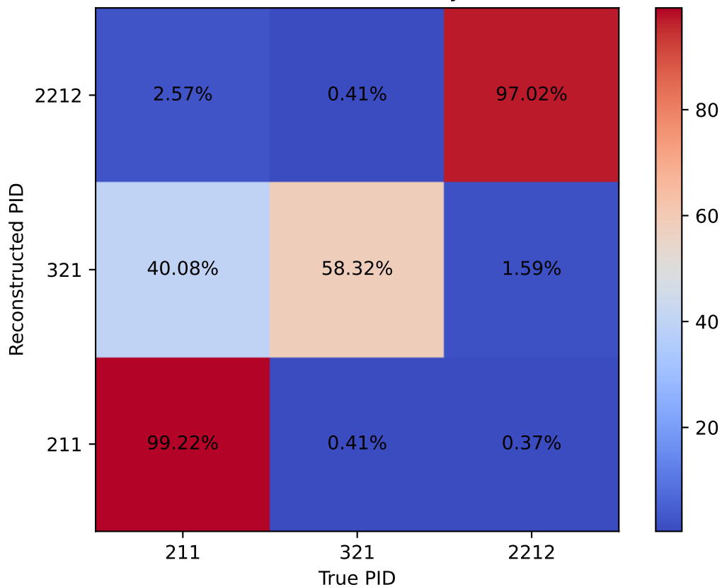
Contamination and Purity Matrix
