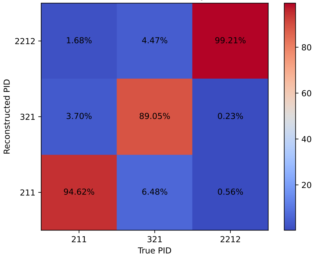
Mis-ID and Efficiency
