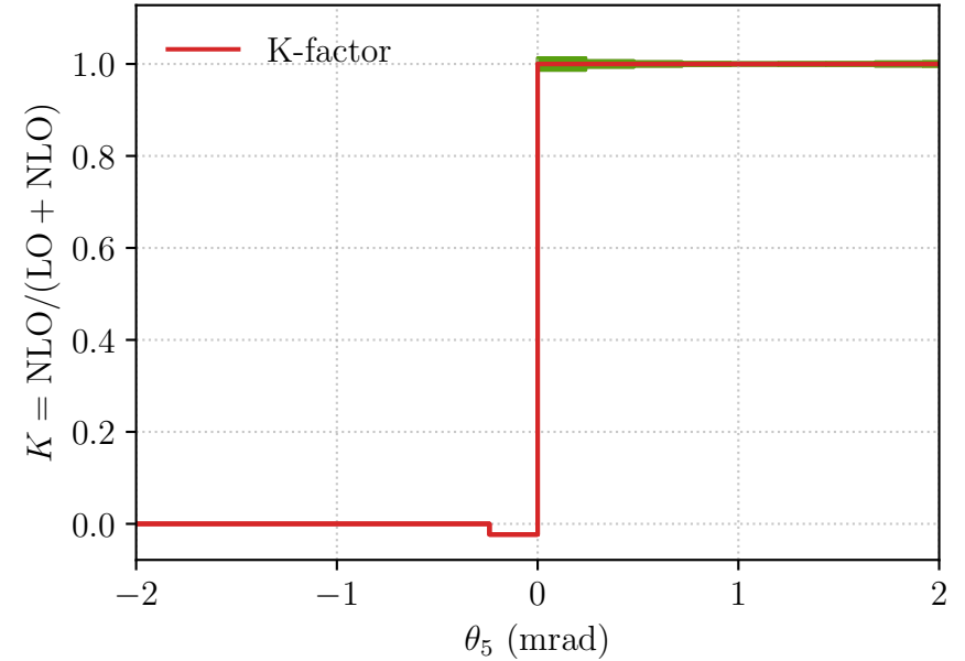
K(\theta_5)
