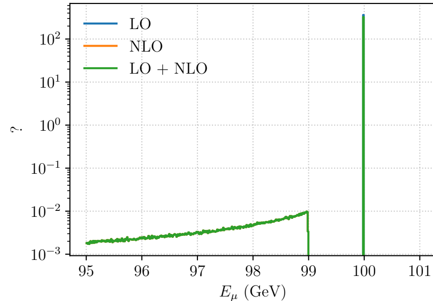
Energy of the Scattered Muon
