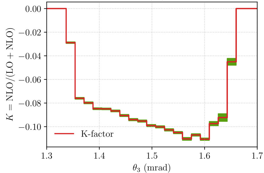
K(\theta_3)
