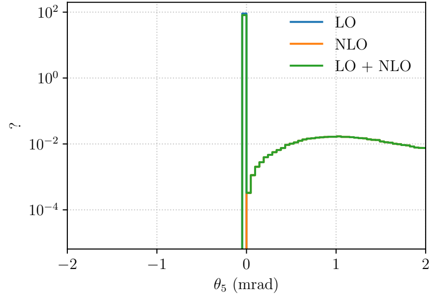
Photon Scattering Angle
