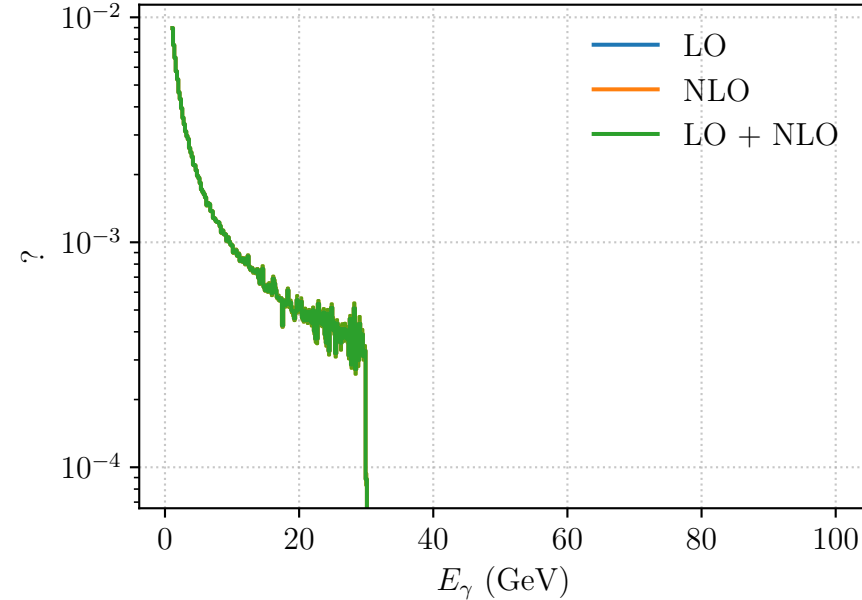
Photon Energy
