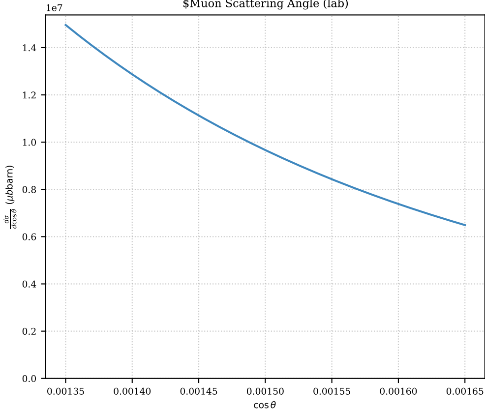
$\mu$on Scattering Angle (lab)
