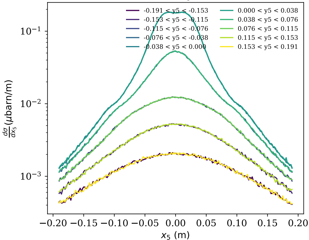
x5 distribution in y5-slices (lab)
