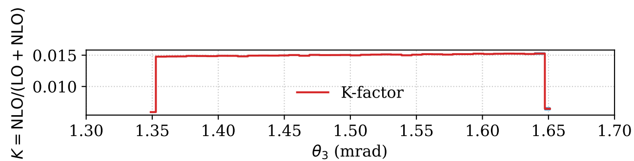
Photon Scattering Angle (lab)
