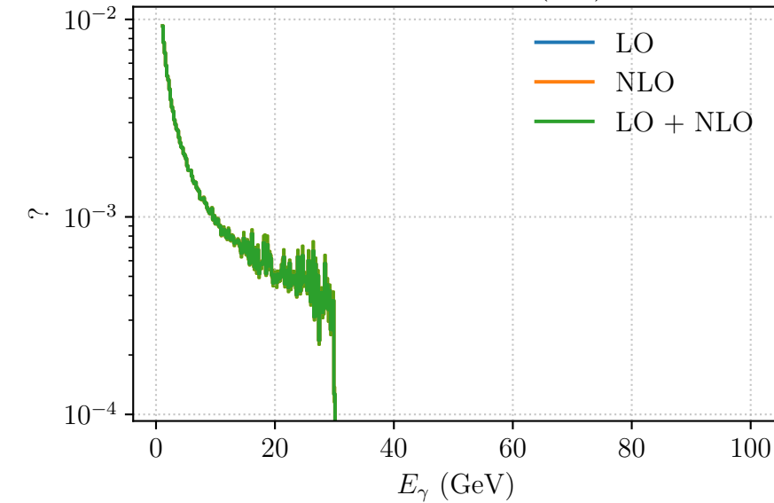
Photon Energy (lab)
