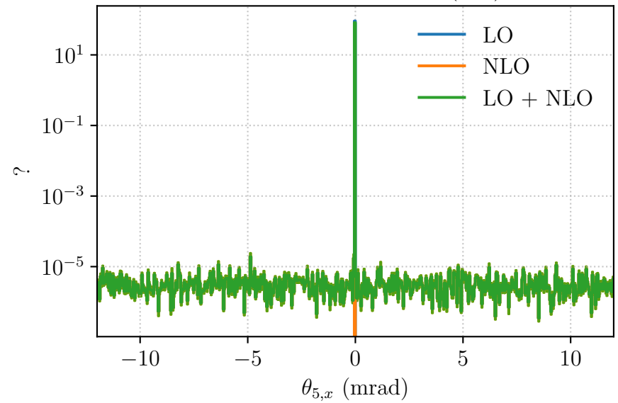
Photon X-deflection (lab)
