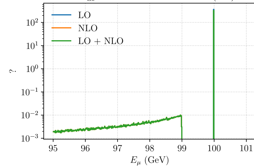
Energy of the Scattered Muon (lab)
