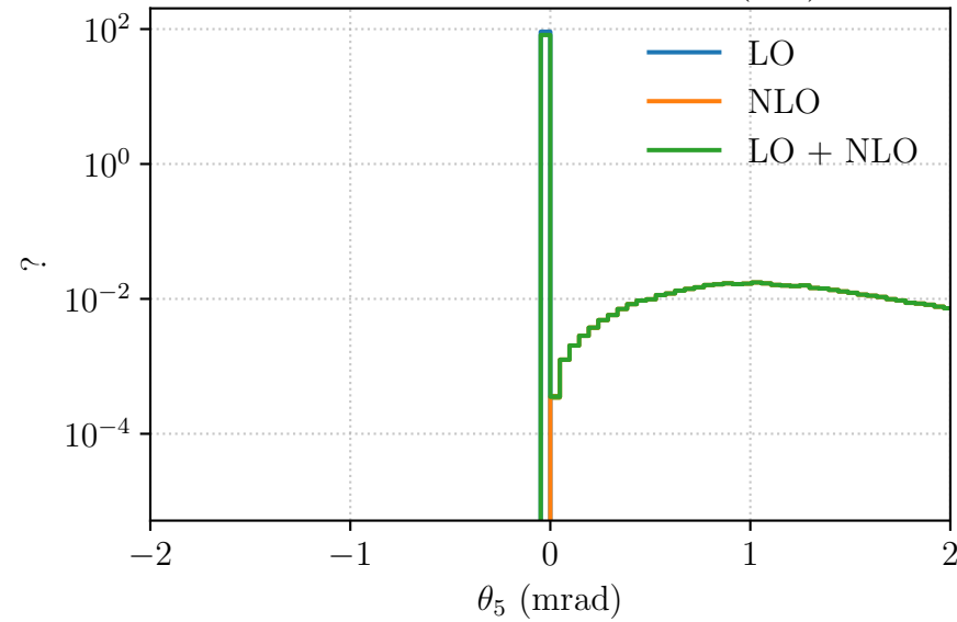
Photon Scattering Angle (lab)
