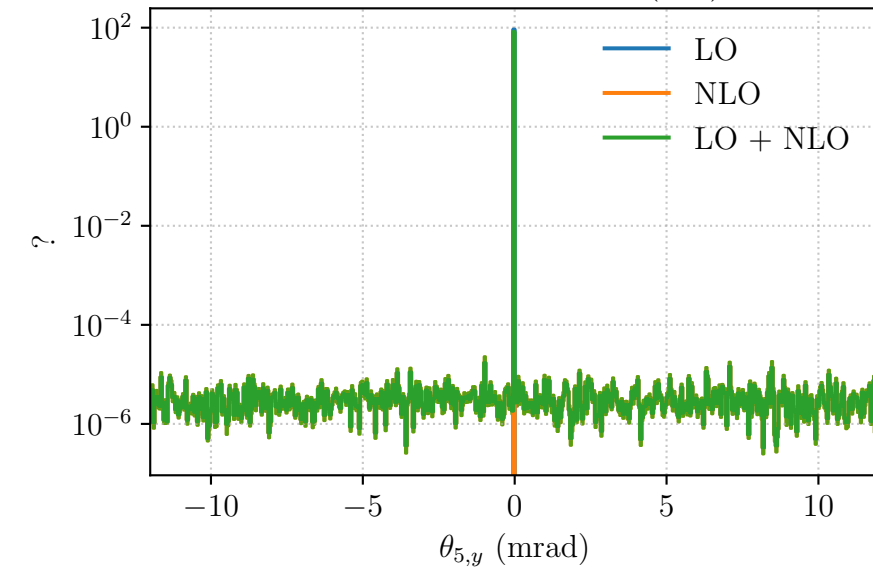
Photon Y-deflection (lab)
