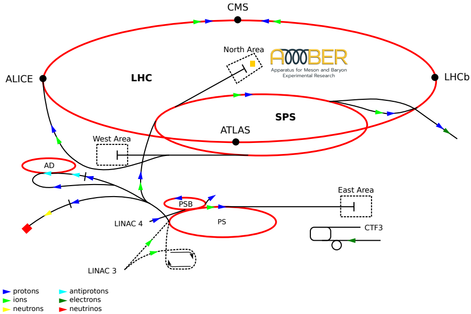
Figure 2.1: Location of the AMBER experiment within the CERN accelerator complex. Figure adapted from [LHC].
