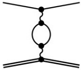
vacuum polarization
