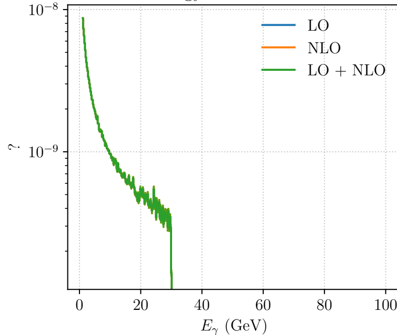
Energy of the Photon
