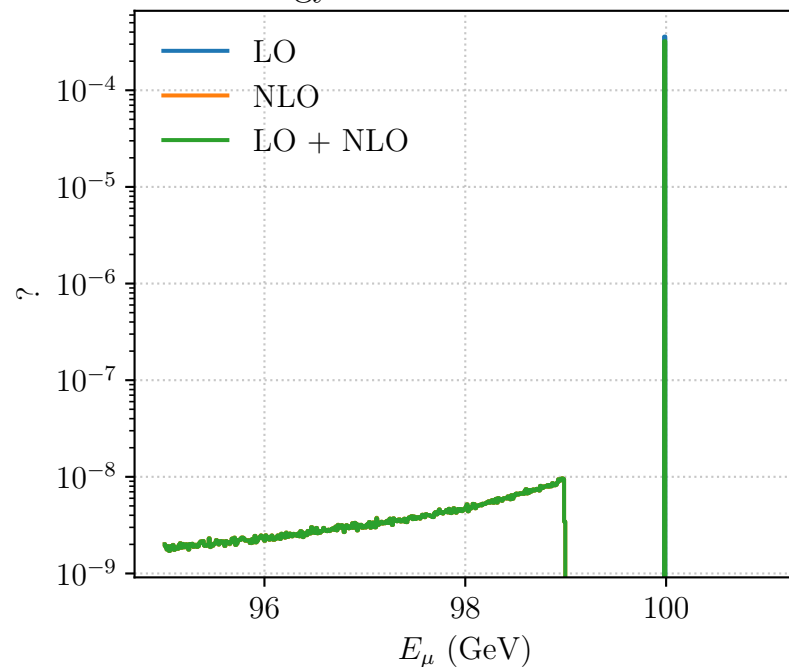
Energy of the Scattered Muon
