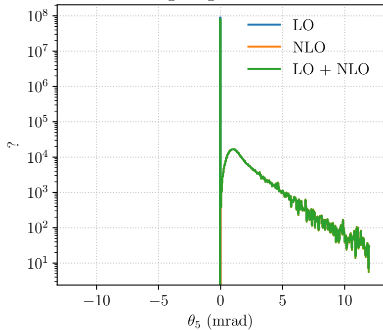
Scattering Angle of the Photon
