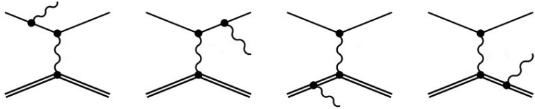
first-order bremsstrahlung processes
