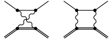
TPE corrections
