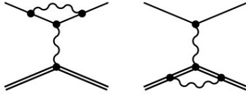
vertex corrections
