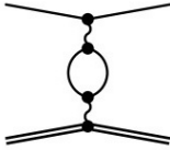
vacuum polarization
