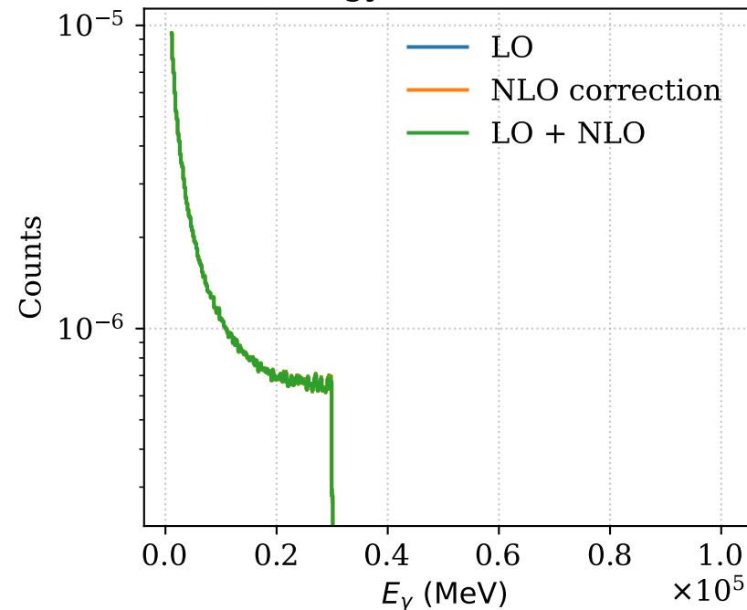
Energy of the Photon
