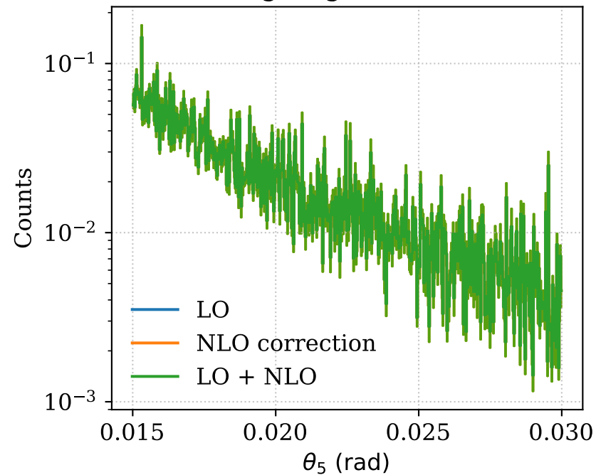
Scattering Angle of the Photon
