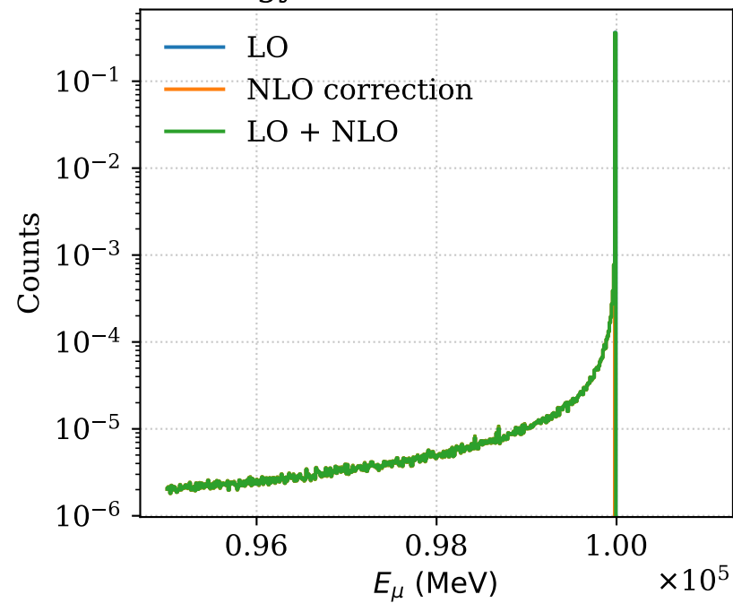
Energy of the Scattered Muon
